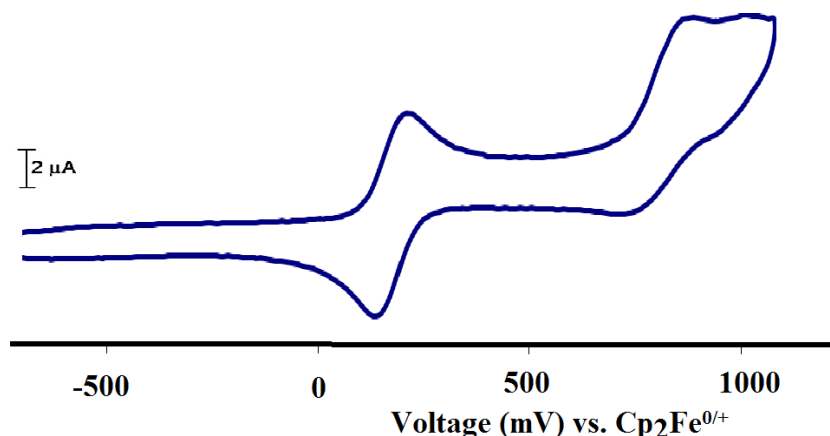
Figure 8. Cyclic voltammograms of complex 1 Data reported in mV vs. \text{Cp}_2\text{Fe}^{0/+} (Pt-disk electrode with A = 0.0064 cm 2 , tetra- n -butylammonium hexafluorophosphate TBAHF, 0.1 M, \text{CH}_2\text{Cl}_2 at 25 °C, scan rate = 0.2 V/s).
