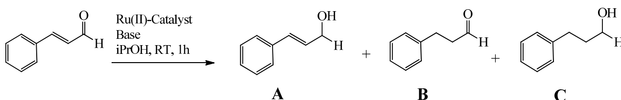
Scheme 2. Different hydrogenation possibilities of cinnamaldehydes: Selective carbonyl group hydrogenation to produce A, selective C=C hydrogenation to produce B, full hydrogenation path with no selectivity to produce C.
