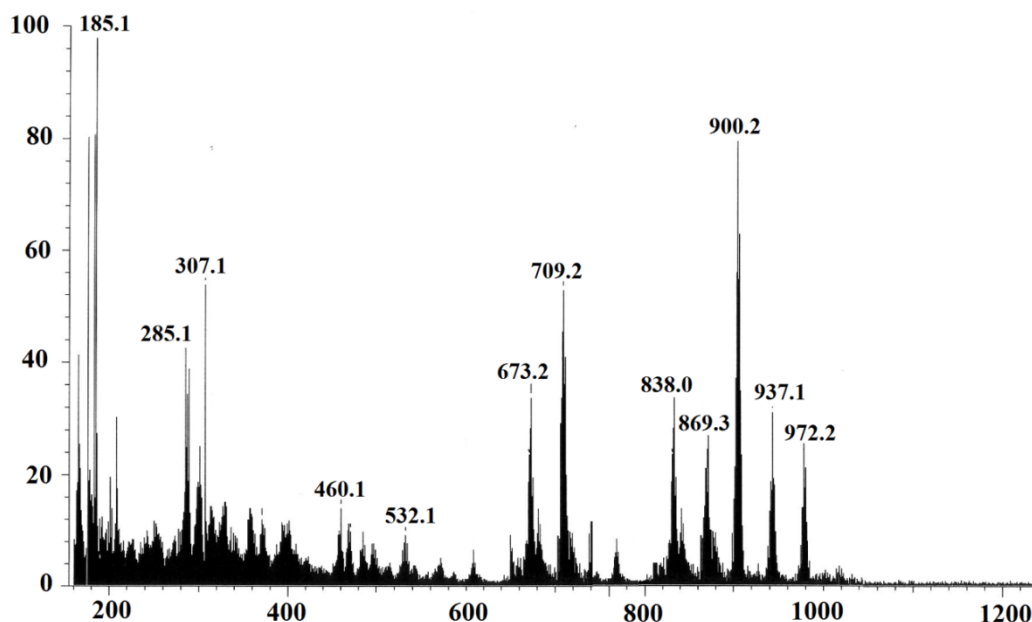
Figure 2. FAB-MS spectrum of complex 1 .
