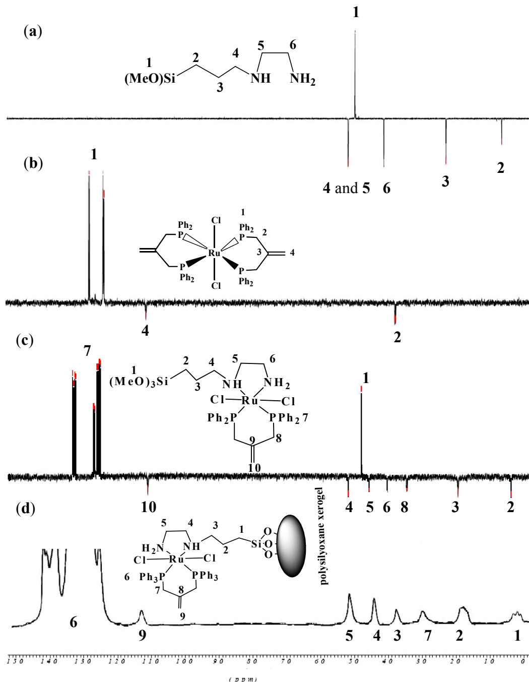
Figure 6. Dept 135^{13}\text{C} -NMR: (a) free [3-(2-aminoethyl)aminopropyl]trimethoxysilane, (b) [\text{RuCl}_2(\text{dppme})_2] , (c) complex 1 , (d) solid state ^{13}\text{C} -CP-MAS-NMR X1 xerogel.
