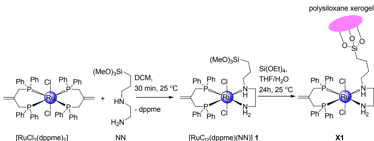
Scheme 1. Synthesis of complex 1 and X1 .
