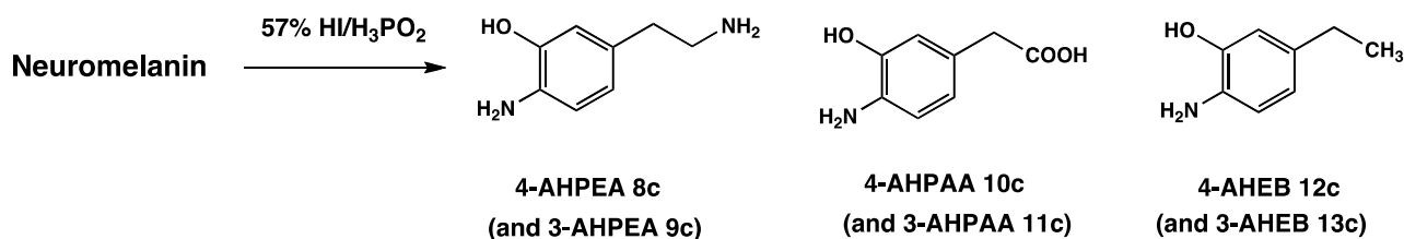
Scheme 2. Possible degradation products afforded by the reductive HI hydrolysis of human NM.
