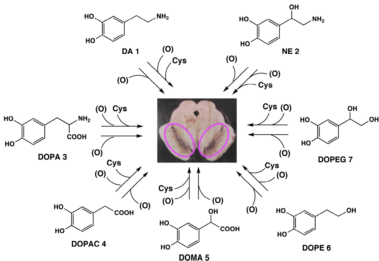
Scheme 2. Possible degradation products afforded by the reductive HI hydrolysis of human NM.
