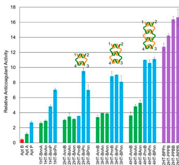
Figure 5. Relative anticoagulant activity of weave tile constructs. Weave tiles with B-P aptamer pairs (blue) demonstrate much better anticoagulant activity compared to those with B-A pairs (green). Activity increases with tile size, except for 2HT-BnPn which shows better activity than 3HT-BnPn. Incorporating multiple copies of Apt P on 2HT-BnPn improves anticoagulation due to higher local concentration (purple). However, incorporating multiple copies of both Apt P and B yields the most effective anticoagulants in 2HT-PPBB and 2HT-BPPB. Weave tile construct names bear a 4-tuple that provides the aptamer identity or “n” for no aptamer for each of the four numbered strand ends (a more thorough explanation of this nomenclature is provided in Section 4.2). Relative anticoagulant activity is calculated as described in Materials and Methods. Error bars represent SEM. Raw clotting times are provided in the Supplementary Materials (Table S2). Relative anticoagulant activity of free aptamer samples is shown for Apt B (red), Apt A (green) and Apt P (blue).
