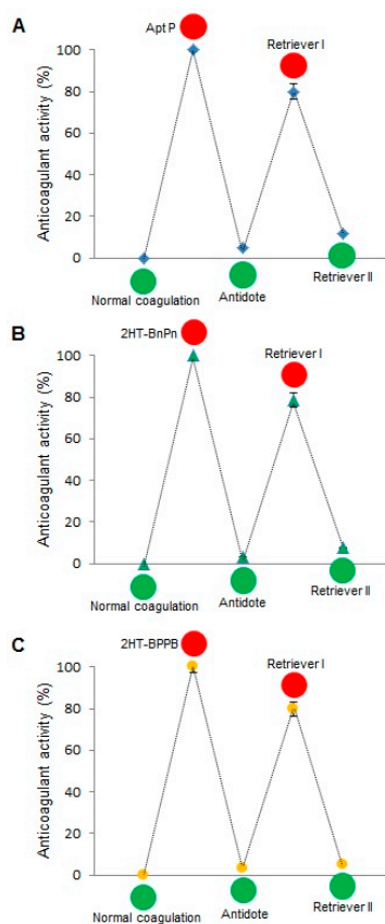
Figure 7. Cycles of antidote/retriever regulation in aPTT assays using (A) Apt P; (B) 2HT-BnPn and (C) 2HT-BPPB. Addition of antidote reverses anticoagulation to less than 10%, whereas addition of retriever I restores it to almost 80%. Retriever II reverses anticoagulation back to less than 10%. The % anticoagulant activity is calculated as described in Materials and Methods. Error bars represent SEM. Raw clotting times are provided in the Supplementary Materials (Table S4).
