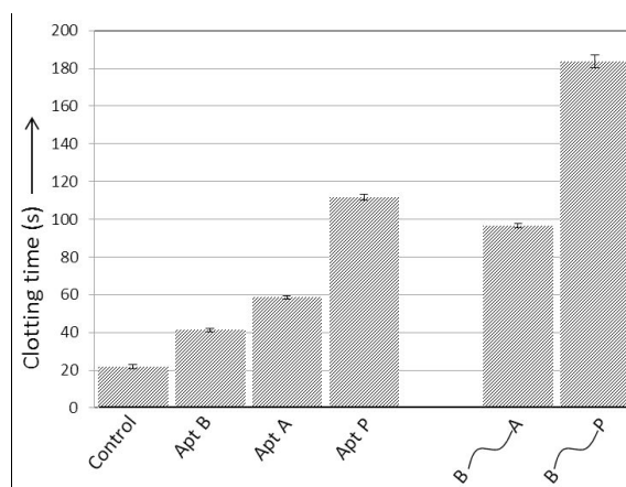
Figure 3. Anticoagulant activity of thrombin-binding aptamers. Apt P demonstrates much better anticoagulant activity than Apt A. Anticoagulant activity improves when the aptamers are linked via a 20-base ssDNA linker, with the B-P pair showing much better anticoagulation than the B-A pair. The concentration of construct in each case is 1 \mu M. Clotting time is expressed as mean \pm SEM.
