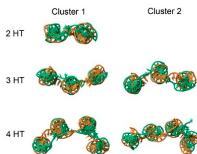
Figure 4. Snapshots showing representative structures of the first two conformational clusters from MD trajectories of weave tiles. According to the clustering metric used, 2HT had a total of 1 cluster, the 3HT had 5 and the 4HT had 7. The first cluster (Cluster 1) is the most common conformation of the tile, while Cluster 2 is the second most common conformation observed during simulations.
