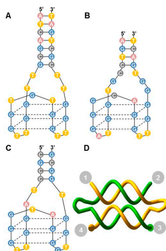
Figure 2. Thrombin-binding aptamers and DNA weave tile. (A) Apt A (also named HD1) with a 7-bp stem and -TT- linkers at the ends; (B) Apt B (also named HD22); (C) Apt P (also called NU172). The structure shown is a model due to the absence of a published crystal structure; (D) A two-helix weave tile (2HT) with the four ends numbered for aptamer positioning and assembly naming.
