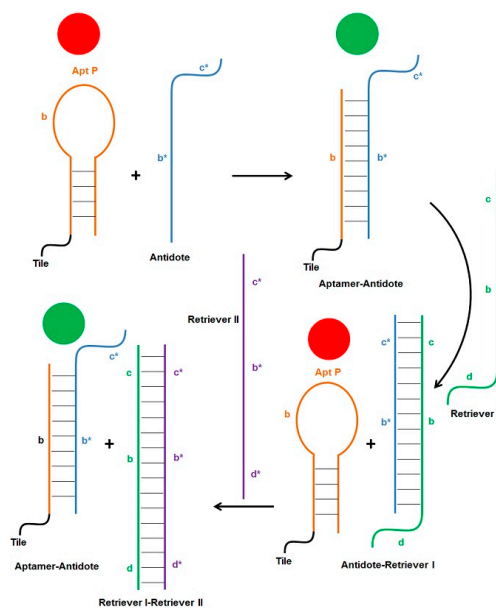
Figure 6. Schematic of regulation cycles. Aptamer turns off the coagulation cascade (red circles), while antidote reverses inhibition and turns on coagulation (green circles). Coagulation can be turned off again by addition of retriever I strand which binds to the overhang in the antidote and displaces the aptamer, which regains its folded structure and inhibits thrombin. Similarly, retriever II strand can displace antidote using the overhang on retriever I. The now free antidote, once again, binds to and deactivates aptamer, turning coagulation back on.
