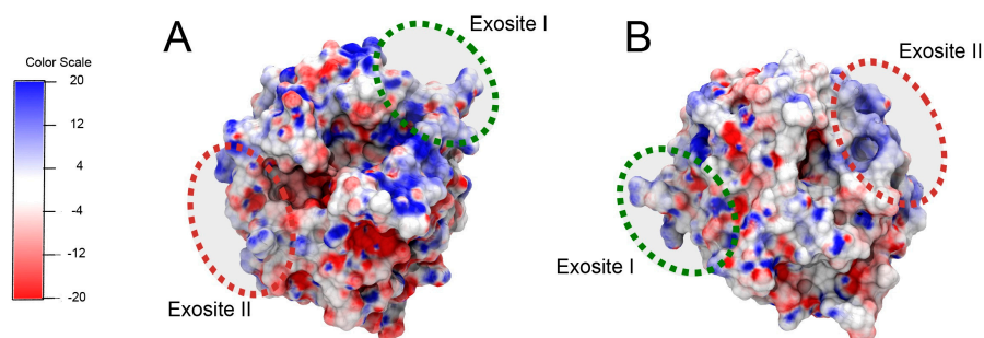
Figure 1. Thrombin structure (pdbID: 1ppb) [4]. (A,B) present two views of the protein. The binding sites of the aptamers (exosites I and II) are highlighted with green and red circles, respectively. Thrombin's surface is colored by electrostatic potential, where red corresponds to negative potential and blue corresponds to a positive potential (units are kT/e ) [5–7].
