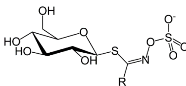
Figure 1. Structure of glucosinolates, where R is the variable side chain from amino acids [9].
