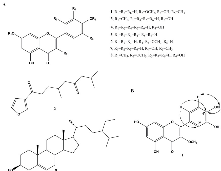
Figure 1. Compounds isolated from M. bontioides . (A) Chemical structures of compounds 1–9 ; and (B) key HMBCs ( \text{H} \rightarrow \text{C} ) and selected NOESY ( \text{H} \leftrightarrow \text{H} ) correlations of compound 1 .
