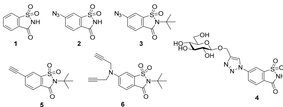
Figure 1. Saccharin 1 , 6-azidosaccharin 2 , N - t -butyl protected 6-azidosaccharin 3 , derivatised saccharin glycoconjugate 4 [10], and new saccharin alkyne building blocks 5 and 6 .
