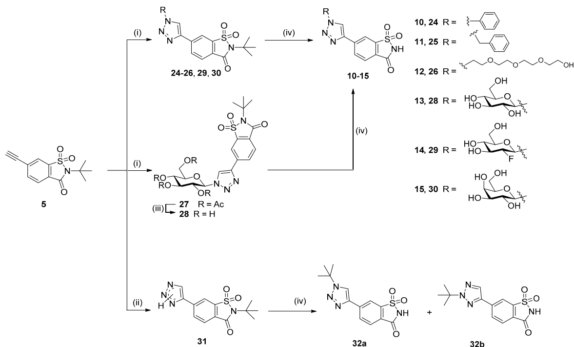
Scheme 2. Synthesis of saccharin derivatives from N - t -butyl-protected 6-ethynylsaccharin 5 . Reagents and conditions: (i) 5 (1 equiv), azide (1 equiv), sodium ascorbate (0.4 equiv), CuSO 4 ·5H 2 O (0.2 equiv), 1:1 t -BuOH:water, 45–50 °C, 2 h–overnight; (ii) 5 (1 equiv), TMSN 3 (2 equiv), sodium ascorbate (0.4 equiv), CuSO 4 ·5H 2 O (0.2 equiv), 1:1 t -BuOH:water, 45–50 °C, overnight; (iii) 8% HCl in MeOH, r.t., 90 h; (iv) TFA, reflux, 18 h.
