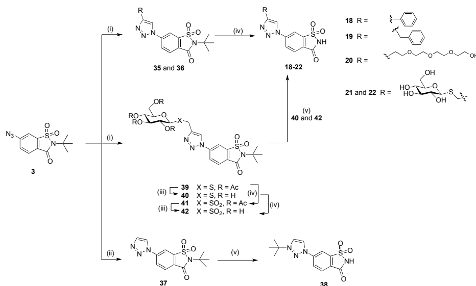
Scheme 4. Synthesis of saccharin derivatives from N - t -butyl-protected 6-azidosaccharin 3 . Reagents and conditions: (i) 3 (1 equiv), alkyne (1 equiv), sodium ascorbate (0.4 equiv), \text{CuSO}_4 \cdot 5\text{H}_2\text{O} (0.2 equiv), 1:1 t -BuOH:water, 45 °C–50 °C, 2 h—overnight; (ii) 3 (1 equiv), TMS-CH (2 equiv), sodium ascorbate (0.4 equiv), \text{CuSO}_4 \cdot 5\text{H}_2\text{O} (0.2 equiv), 1:1 t -BuOH:water, 45 °C, overnight; (iii) 8% HCl in MeOH, r.t., 90 h; (iv) m CPBA, \text{CH}_2\text{Cl}_2 , 0 °C to r.t.; (v) TFA, reflux, 18 h. The phenyl derivative 18 as previously reported [10].
