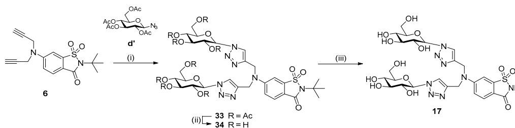
Scheme 3. Synthesis of saccharin glycoconjugate 17 from bis-alkyne 6 . Reagents and conditions: (i) \text{CuSO}_4 \cdot 5\text{H}_2\text{O} (0.2 equiv), 1:1 t -BuOH:water, 45 °C, 87%; (ii) 8% HCl in MeOH, r.t., 90 h, 92%; (iii) TFA, reflux, 18 h, 84%.
