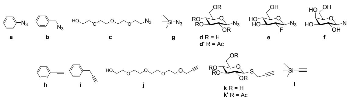
Figure 2. Partner azides ( a–g ) and alkynes ( h–l ) for preparing derivatives of 1 using Cu(I)-catalyzed azide alkyne cycloaddition (CuAAC).
