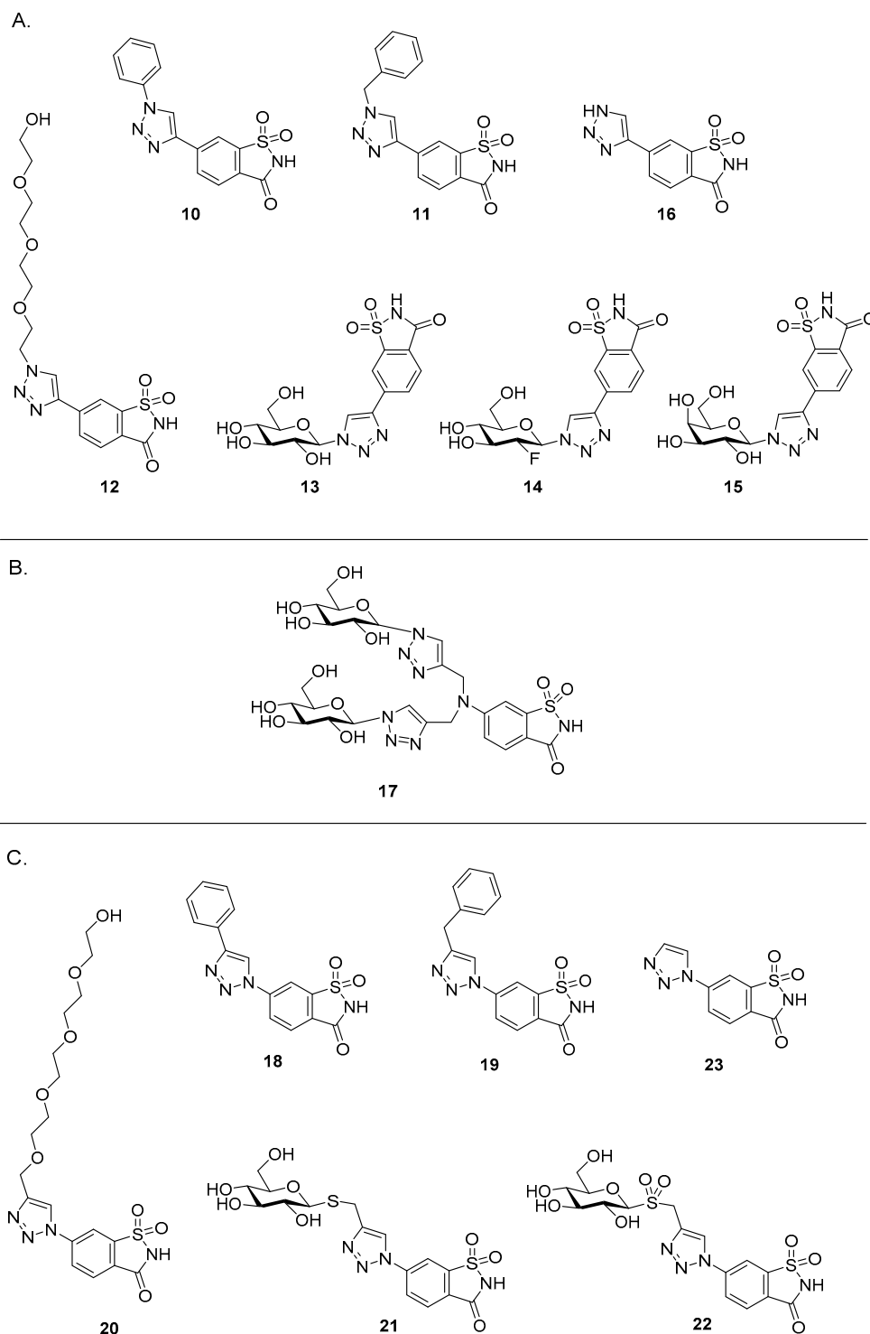
Figure 3. Target derivatives of 1 prepared using CuAAC. (A) Derivatives prepared from N - t -butyl-protected 6-ethynylsaccharin 5 and azide a–g ; (B) Derivative prepared from N - t -butyl-protected bis-alkyne saccharin 6 and azide d/d' ; (C) Derivatives prepared from N - t -butyl-6-aminosaccharin 7 and alkynes h–l . We have previously reported the phenyl derivative 18 while all other compounds are novel [10].
