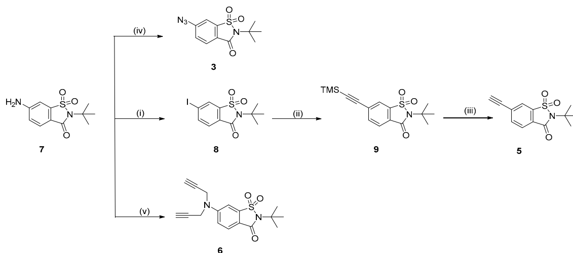
Scheme 1: Synthesis of N - t -butyl-protected 6-azidosaccharin 3 [10], N - t -butyl-protected 6-ethynylsaccharin 5 , and N - t -butyl-protected bis-alkyne saccharin 6 . Reagents and conditions: (i) p\text{TsOH}\cdot\text{H}_2\text{O} , \text{NaNO}_2 , KI, \text{CH}_3\text{CN} , 10\text{--}15\text{ }^\circ\text{C} \rightarrow \text{rt} , ~1 h, 83%; (ii) \text{Pd}(\text{PPh}_3)_2\text{Cl}_2 , \text{CuI} , \text{TMS-C}\equiv\text{CH} , \text{Et}_3\text{N} , 40\text{ }^\circ\text{C} , 2 h, 95%; (iii) TBAF, AcOH, THF, 5 min, rt, 97%; (iv) t\text{-BuNO}_2 , \text{TMSN}_3 , 0\text{ }^\circ\text{C} \rightarrow \text{rt} , 16 h, 46% [10]; (v) \text{Cs}_2\text{CO}_3 , propargyl bromide, dimethylformamide (DMF), 0\text{ }^\circ\text{C} , 48 h, 75%.
