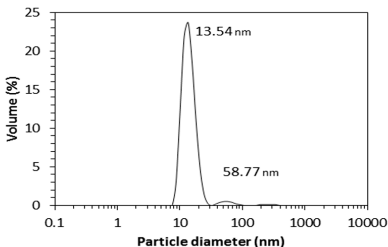
Figure 18. Particle size distribution of the JPU dispersion.
