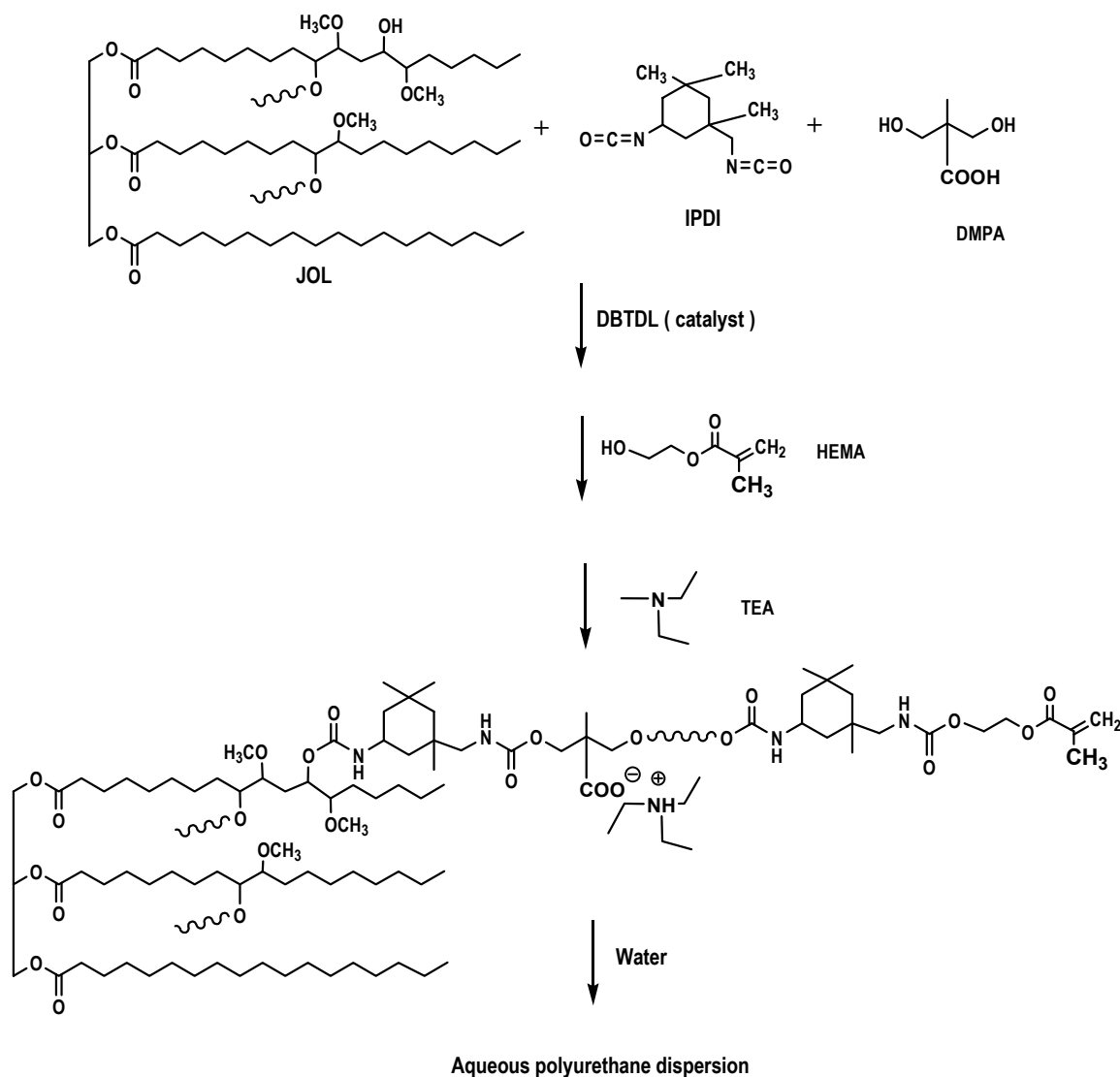
Figure 19. Synthesis of aqueous polyurethane dispersion.
