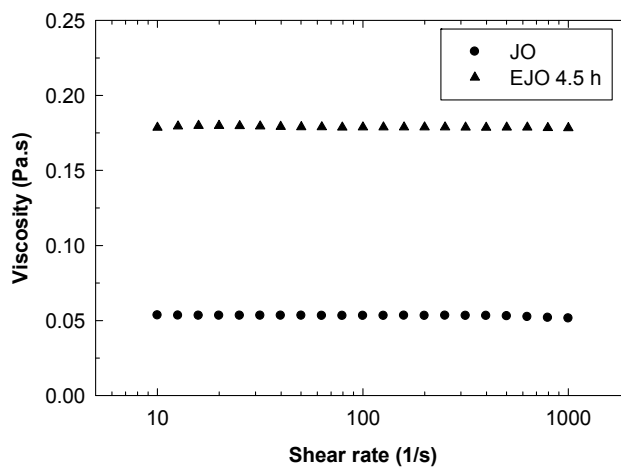
Figure 12. Viscosity curve of jatropha oil (JO) and epoxidised jatropha oil (EJO) at 25 °C.
