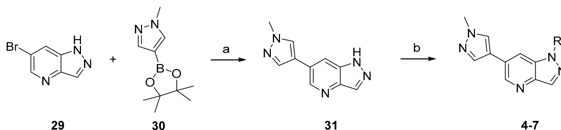
Scheme 1. The synthesis route of compounds 4–7 . Reagents and conditions: (a) Pd(dppf)Cl 2 , K 2 CO 3 , Dioxane:H 2 O ( v/v = 4:1), 80 °C, 2 h, 86% yield; (b) NaH, Dimethylformamide (DMF), R-SO 2 Cl, room temperature (r.t.), 1–4 h, 76–83% yield.
