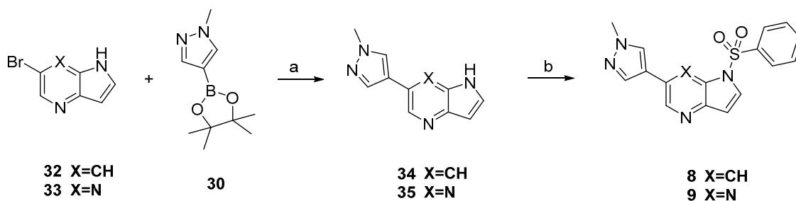
Scheme 2. The synthesis route of compounds 8 and 9 . Reagents and conditions: (a) Pd(dppf)Cl 2 , K 2 CO 3 , Dioxane:H 2 O ( v/v = 4:1), 80 °C, 3 h, 89% yield ( 34 ), 82% yield ( 35 ); (b) NaH, DMF, benzenesulfonyl chloride, r.t., 2 h, 82% yield ( 8 ), 79% yield ( 9 ).
