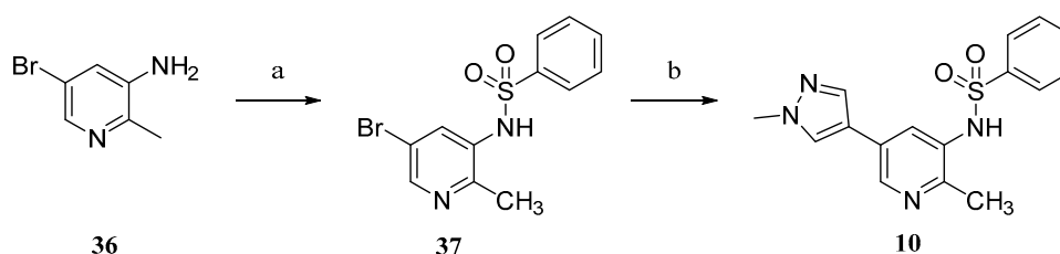
Scheme 3. The synthesis route of compound 10 . Reagents and conditions: (a) benzenesulfonyl chloride, NaH, DMF, r.t., 85% yield; (b) 1-Methylpyrazole-4-boronic acid pinacol ester, Pd(dppf)Cl 2 , K 2 CO 3 , Dioxane:H 2 O ( v/v = 4:1), 80 °C, 3 h, 80% yield.
