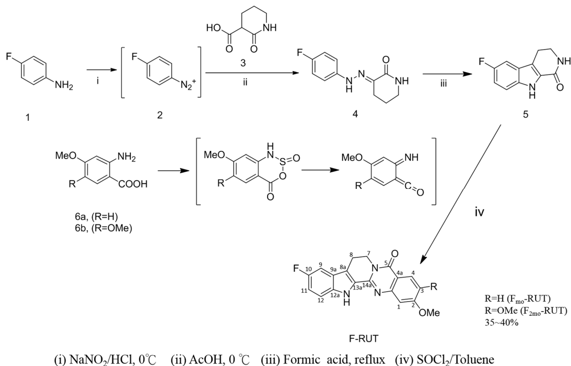
Scheme 1. Synthesis of 10-fluoro-2-methoxyrutaecarpine (F-RUT) and 10-fluoro-2,3-dimethoxyrutaecarpine.
