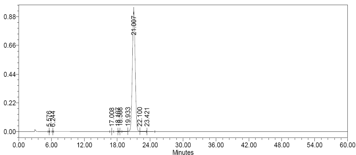
Figure 5. The purity of SAG detected by HPLC. SAG was analyzed by HPLC with UV detection at 204 nm. The analysis was performed with a C-18 column (4.6 mm \times 250 mm) at 35 °C. It was eluted (eluent A: acetonitrile; eluent B: 0.2% phosphate solution) at a flow rate of 1.0 mL/min.
