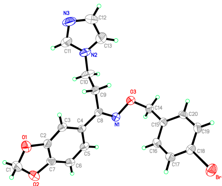
Figure 2. ORTEP diagram of compound Vi . Displacement ellipsoids are plotted at the 40% probability level for non-H atoms.
