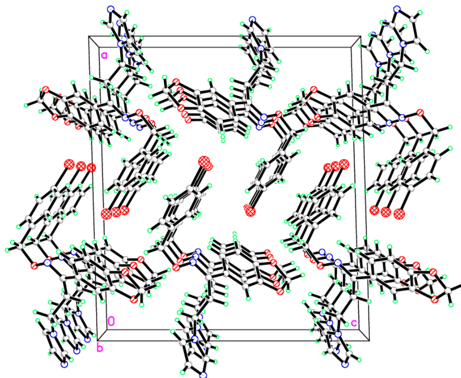
Figure 3. Molecular packing of compound Vi.
