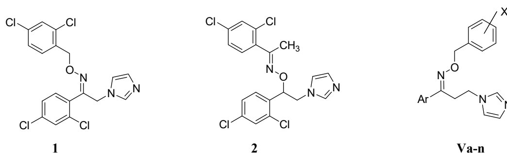
Figure 1. Chemical structures of the antifungal agents 1 and 2 as well as the target compounds Va–n .
