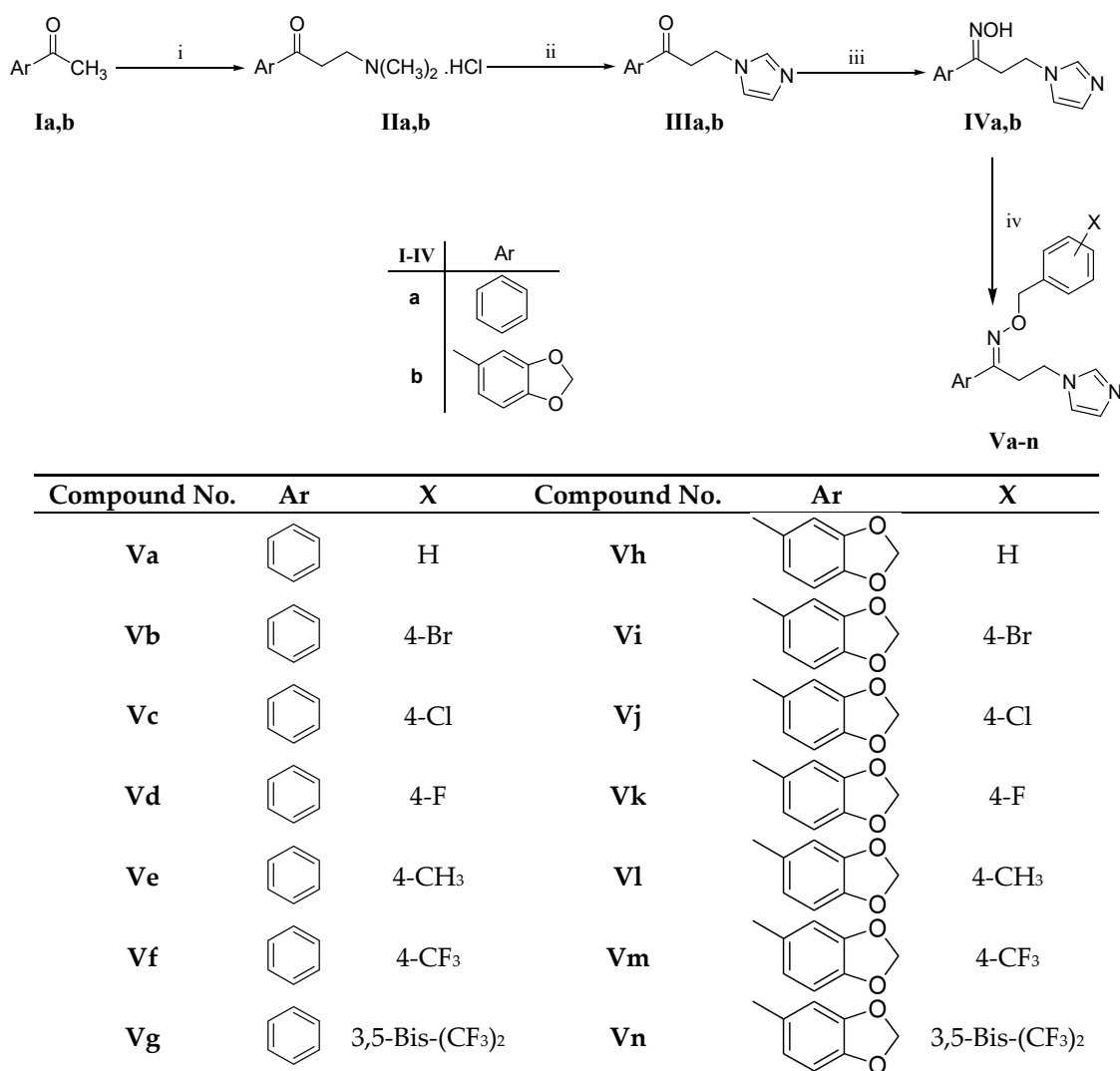
Scheme 1. Synthesis of the target compounds Va–n . Reagents and conditions: (i) \text{HN}(\text{CH}_3)_2 \cdot \text{HCl} , (\text{CH}_2\text{O})_n , conc. \text{HCl} , ethanol, reflux, 2 h; (ii) Imidazole, water, reflux, 5 h; (iii) \text{H}_2\text{NOH} \cdot \text{HCl} , \text{KOH} , ethanol, reflux, 18 h; (iv) Appropriate benzyl chloride/bromide derivative, \text{NaH} , \text{DMF} , 80^\circ\text{C} , 3 h.
