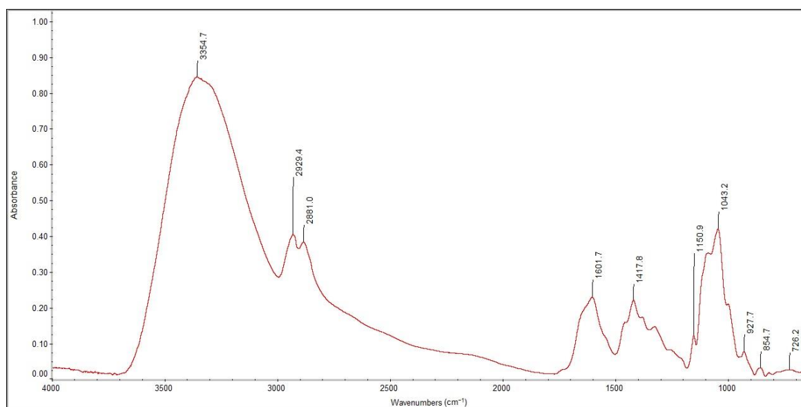
Figure 7. Fourier Transform Infrared Study (FTIR) spectra of the lyophilized foam before irradiation sterilization.
