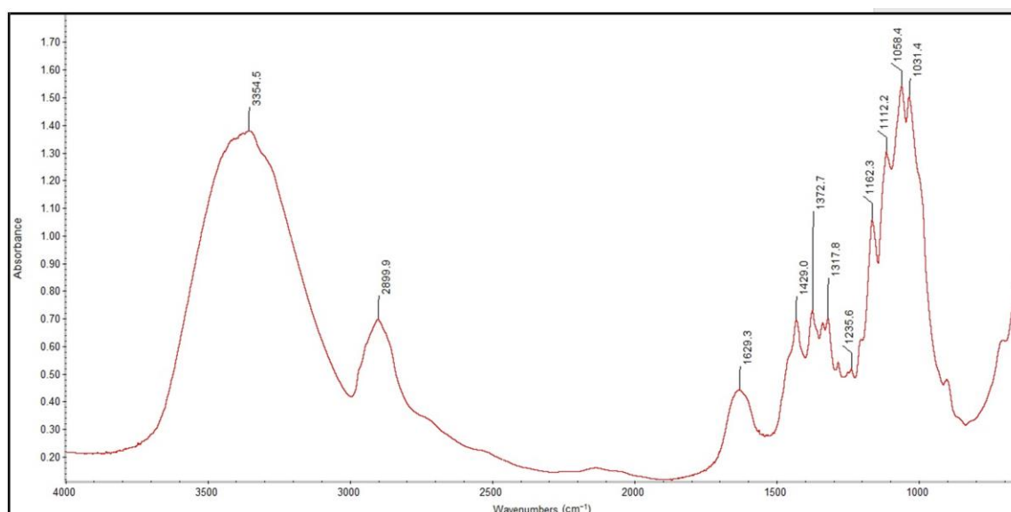
Figure 8. FTIR spectra of the impregnated gauze before irradiation sterilization.
