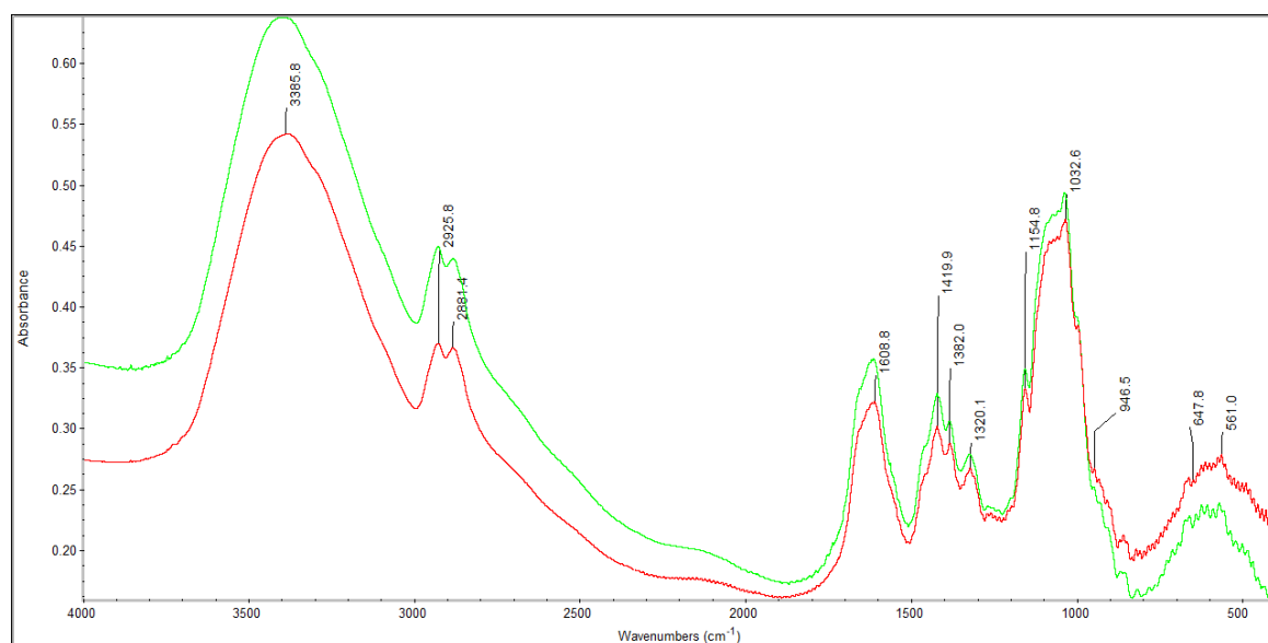
Figure 9. FTIR spectra of the sterilized lyophilized foam before and after the accelerated ageing process: - initial; - after one year of simulated ageing.
