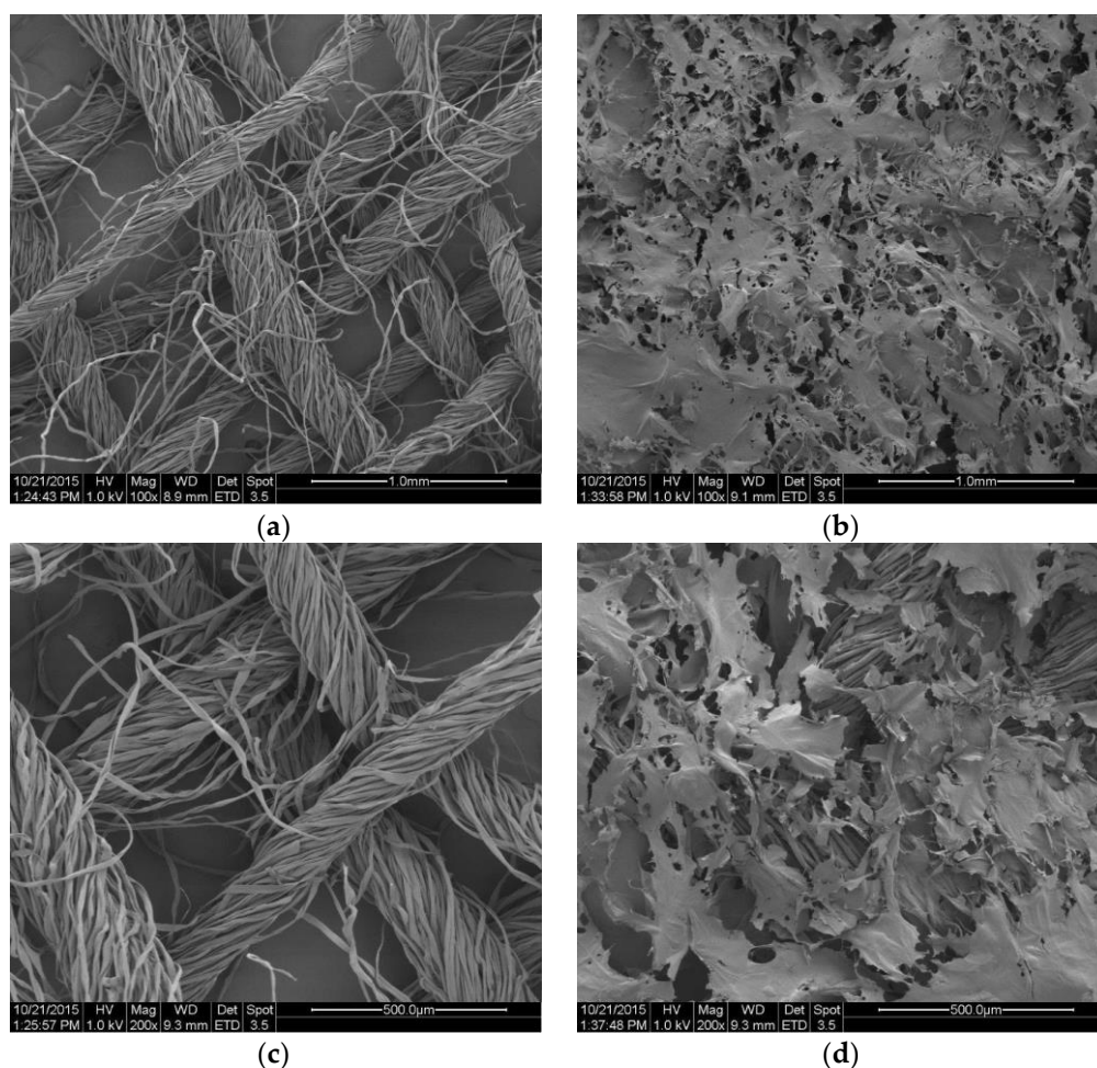
Figure 11. SEM microphotographs of: (a) gauze before impregnation (initial) at magnification 100×; (b) impregnated gauze at magnification 100×; (c) gauze before impregnation (initial at magnification 200×; and (d) impregnated gauze at magnification 200×.
