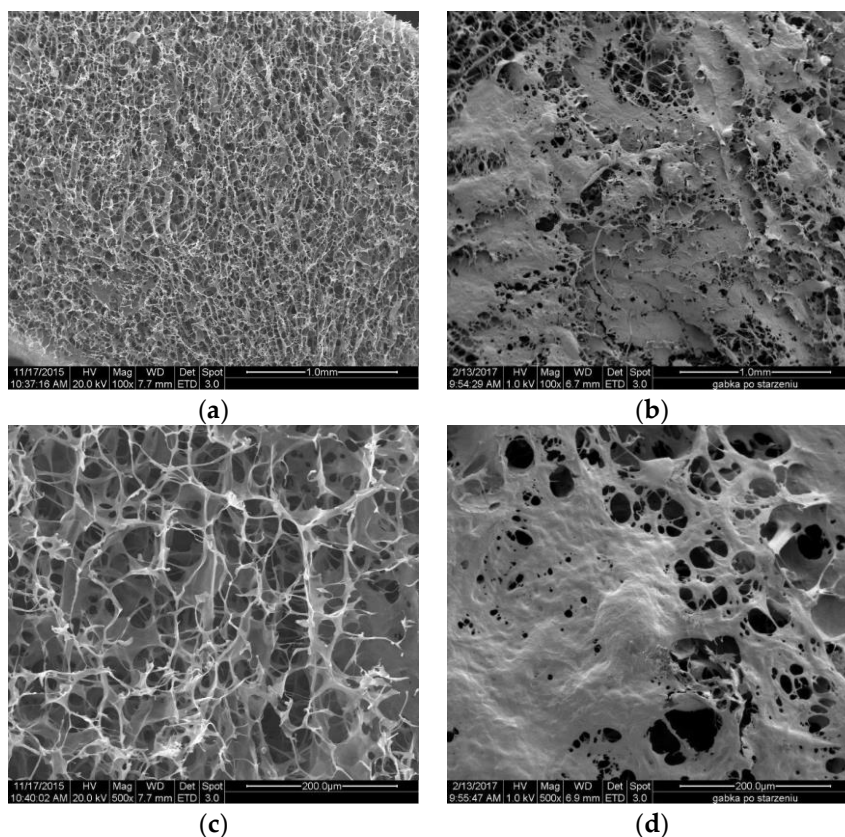
Figure 13. SEM microphotographs of (a) foam before accelerated ageing at magnification 100×; (b) foam after accelerated ageing at magnification 100×; (c) foam before accelerated ageing at magnification 500×; and (d) foam after accelerated ageing at magnification 500×.
