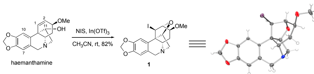
Figure 1. Synthesis of compound 1 and its x-ray structure. Thermal ellipsoids are drawn at the 50% probability level.
