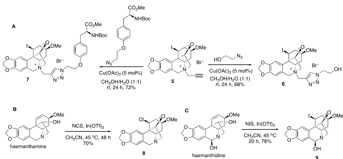
Figure 3. (A) Click reactions of compound 5, (B) chloro variant of the original transformation, and (C) an analogous transformation of alkaloid haemanthidine.
