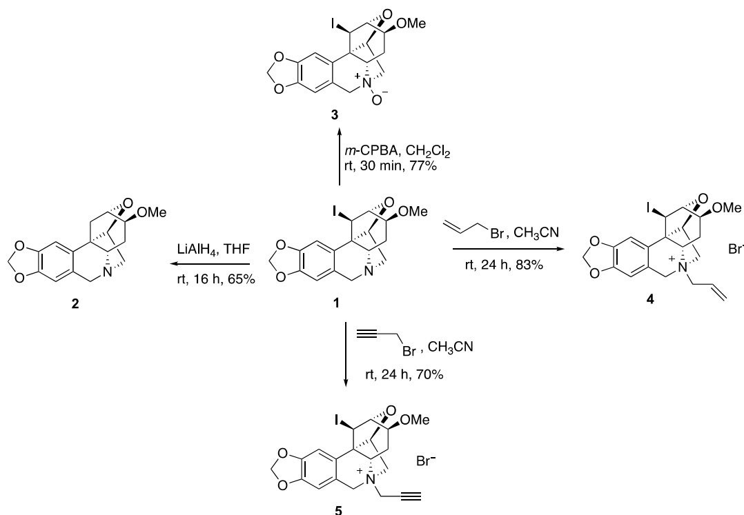
Figure 2. Derivatization of compound 1.
