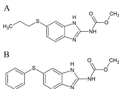
Figure 1. Chemical structures of (A) albendazole and (B) fenbendazole.
