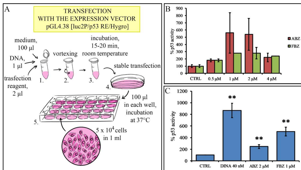
Figure 2. Luciferase assay of A375 melanoma cell line carrying a p53 activity luciferase reporter construct. (A) Scheme of HTS screening of 2448 compounds. (B) HTS revealed albendazole (ABZ) and fenbendazole (FBZ) as compounds that activate p53. (C) ABZ (2 \mu M) and FBZ (1 \mu M) significantly increased the activity of p53, dinaciclib (DINA) (40 nM) was used as a positive control. Solvent (DMSO) treated cells were used as a negative control (CTRL). The data are the means \pm S.E.M. of three independent experiments; ** p < 0.01.
