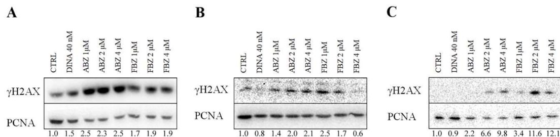
Figure 6. ABZ and FBZ caused DNA damage. WB analysis revealed increased levels of \gamma H2AX in all (A) A375, (B) MCF7, and (C) HFF cells treated with ABZ and FBZ (1, 2, and 4 \mu M) for 24 h. Total cell lysates were separated on a 12.5% SDS gel. PCNA was used as a loading marker. Solvent (DMSO) treated cells were used as a negative control (CTRL). DINA (40 nM) that was used as a positive control affected H2AX phosphorylation only in A375 cells. Numeric values represent the ratio of band densities of the protein of interest normalized to the corresponding PCNA and the control normalized to the corresponding PCNA.
