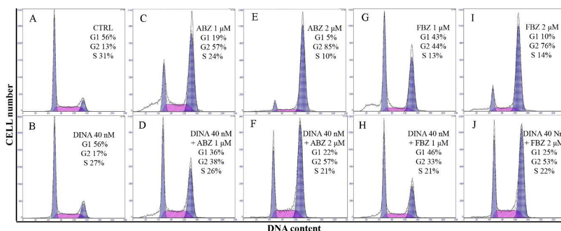
Figure 5. ABZ and FBZ arrest cell cycle at G2/M phase. Flow cytometry analysis of PI-stained cells. (A) Control, DMSO treated cells. (B) Cells treated with DINA. (C,E,G,I) ABZ and FBZ (1 and 2 \mu M) and their combinations with DINA (40 nM, D,F,H,J) significantly increased the proportion of A375 cells in G2/M phase. DINA alone had no significant effect on the cell cycle distribution.
