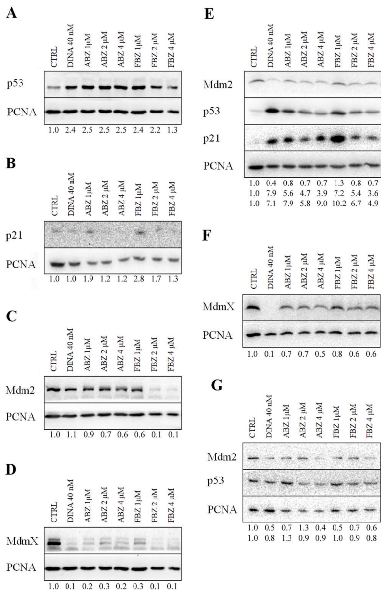
Figure 3. Effect of benzimidazoles on p53 and related proteins levels. DINA (40 nM) was used as a positive control. Solvent (DMSO)-treated cells were used as a negative control (CTRL). (A–D) WB analysis of A375 cells. (A) The A375 cells treated 24 h with ABZ (1, 2, and 4 \mu\text{M} ), FBZ (1 and 2 \mu\text{M} ), and DINA (40 nM) revealed p53 stabilization. (B) ABZ (1 \mu\text{M} ) and FBZ (1 \mu\text{M} ) increased the level of p21. (C) FBZ (2 \mu\text{M} and 4 \mu\text{M} ) decreased the level of Mdm2, ABZ at all concentrations and FBZ (1 \mu\text{M} ) had a weaker effect, and DINA did not affect p21. (D) The level of MdmX was decreased upon the treatment with DINA (40 nM), ABZ, and FBZ at concentrations 1, 2, and 4 \mu\text{M} . (E–F) Similar results were also obtained with MCF7 breast carcinoma cells. (E) p53 stabilization, an increase of p21 and
