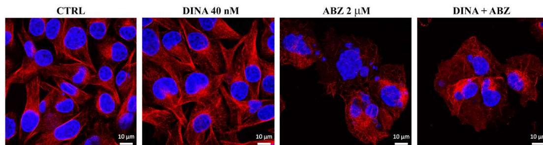
Figure 4. ABZ disrupts microtubules in A375 cells. Confocal laser scanning microscopy. Microtubules (red) stained by indirect immunofluorescence and nuclei (DAPI staining, blue) after 24 h treatment with ABZ (2 \mu M), DINA (40 nM), and a combination of both. The regular network of microtubules in control and DINA-treated cells. Thinned, disappearing, and irregular microtubules and multiple nuclei were apparent in cells treated with ABZ and the combination of ABZ with DINA. Bar = 10 \mu m.
