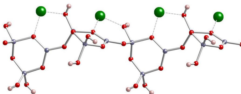
Figure 2. Four repeating units of the polytriborate chain in \text{Zn}[\text{B}_3\text{O}_4(\text{OH})_3] .
