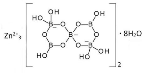
Figure 5. The proposed structure of 3\text{ZnO}\cdot 5\text{B}_2\text{O}_3\cdot 14\text{H}_2\text{O} [17].
