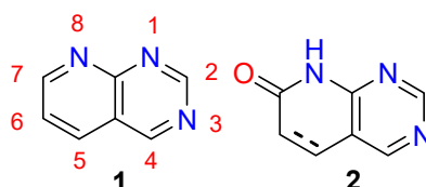
Figure 1. Structures of the pyrido[2,3- d ]pyrimidine ring system ( 1 ) and pyrido[2,3- d ]pyrimidin-7(8 H )-ones ( 2 ).
