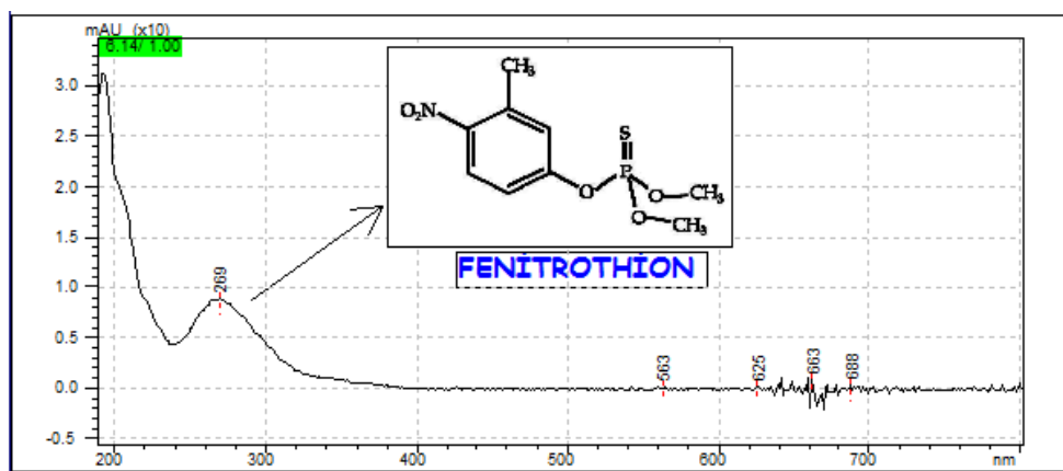
S1. Absorption spectrum of PRO and FEN obtained from DAD detector
