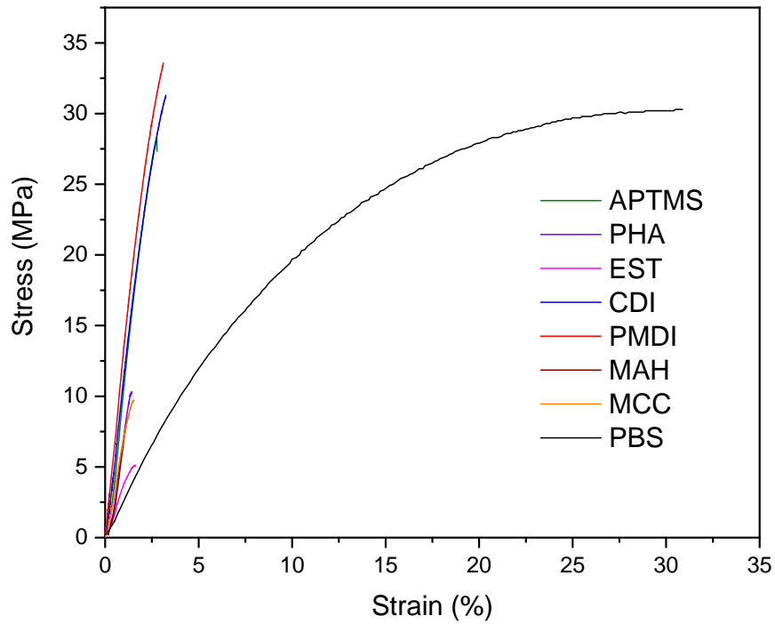
Figure s3. Example of the characteristic tensile curves of PBS/MCC composites.
