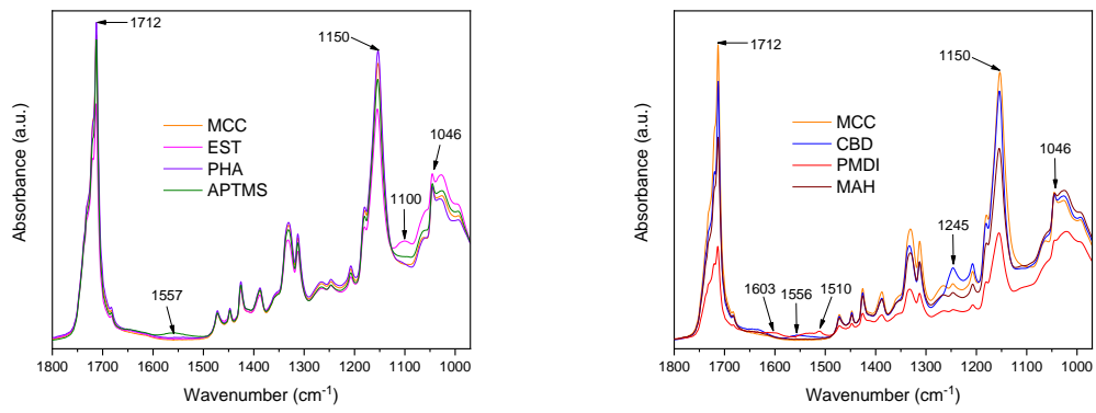
Figure s2. FTIR spectra of PBS/MCC composites.
