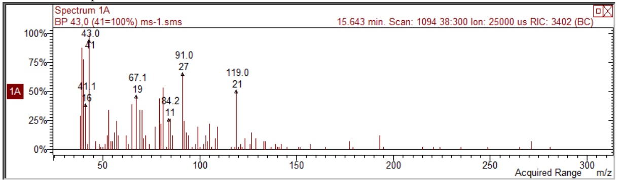
Figure 1 Mass spectra of unidentified VOCs in peppermint aroma profile. Both mass spectra was obtained by GC-MS analysis with Varian CP-3800/Saturn 2000 apparatus (Varian, Walnut Creek, CA, USA). MS operational conditions were as follows: ion source temperature: 250°C; electron impact (EI) ionization at 70 eV; scanning mode from 35 to 300 m/z .
