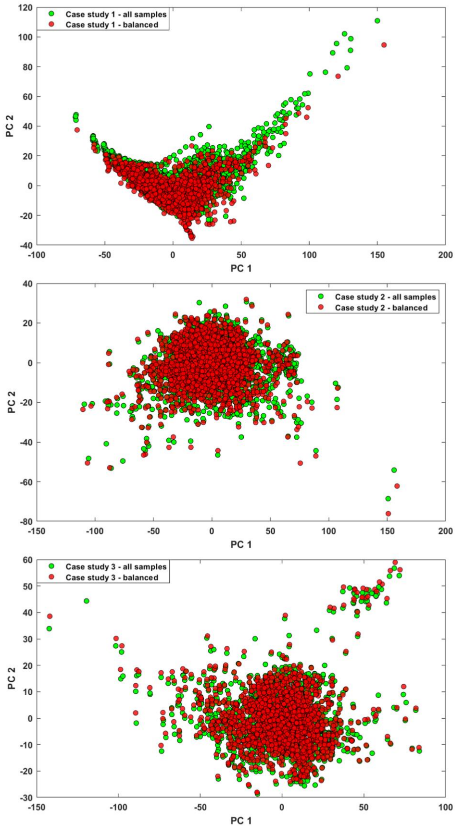
Figure S1. The applied modeling workflow (a). Principal component analysis (PCA) score plots (b).
