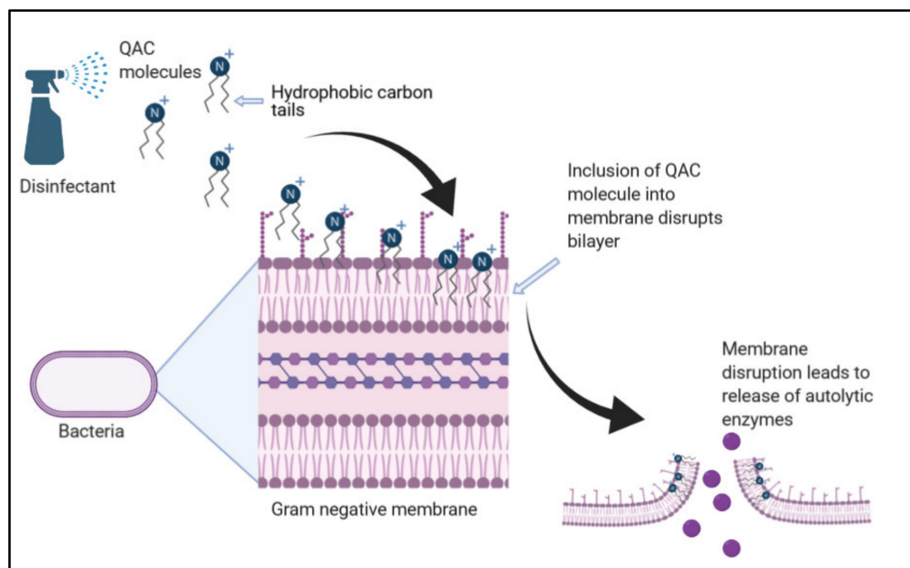
Figure 1. The bactericidal process by quaternary ammonium compound (QAC) disinfectants. The hydrophobic alkyl chains of the QAC salt interact with the phospholipid bilayer. This increases membrane permeability and induces the release of autolytic enzymes, resulting in bacterial cell lysis (adapted from [12,13]).
