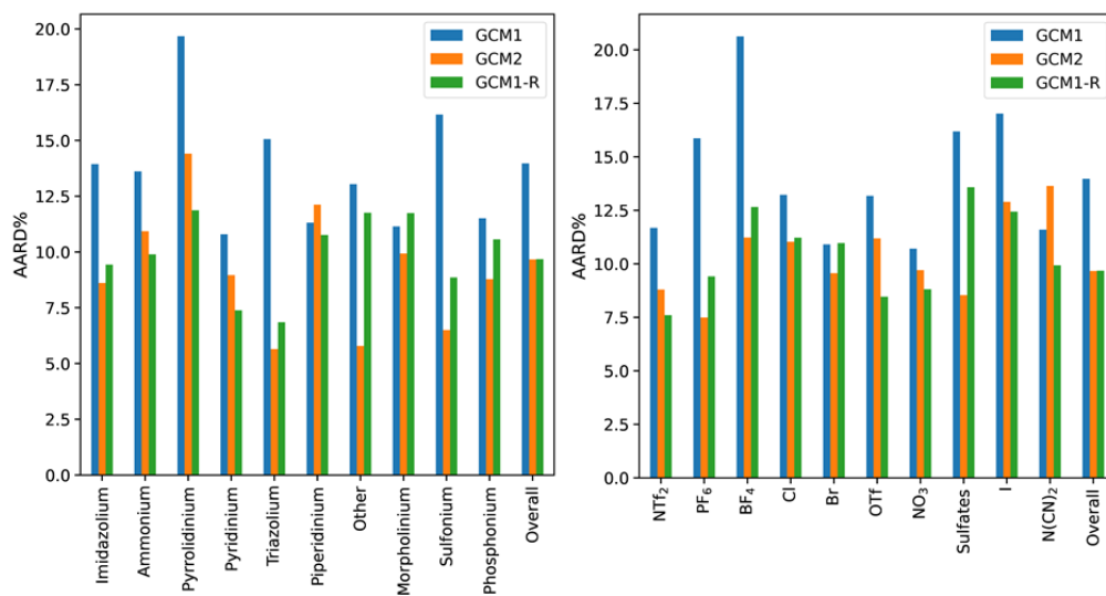
Figure 7. Comparison of AARD for GCM1-R with GCM1 and GCM2 for the estimation of IL melting point according to (a) cation type and (b) anion type.
