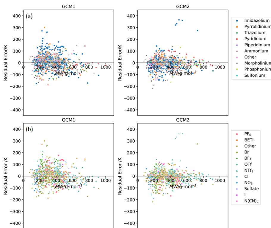
Figure 3. Residual plots of error versus IL molecular weight obtained using GCM1 and GCM2 to estimate melting points for ILs containing the major (a) cation and (b) anion types.
