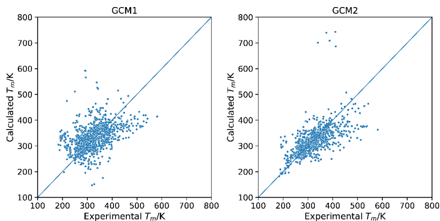
Figure 1. Parity plots of calculated versus experimental melting points for (a) GCM1 and (b) GCM2.
