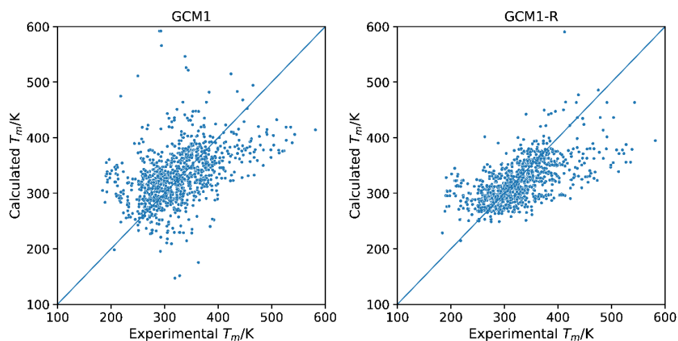
Figure 6. Parity plots of calculated versus experimental melting points for (a) GCM1 and (b) GCM1-R.
