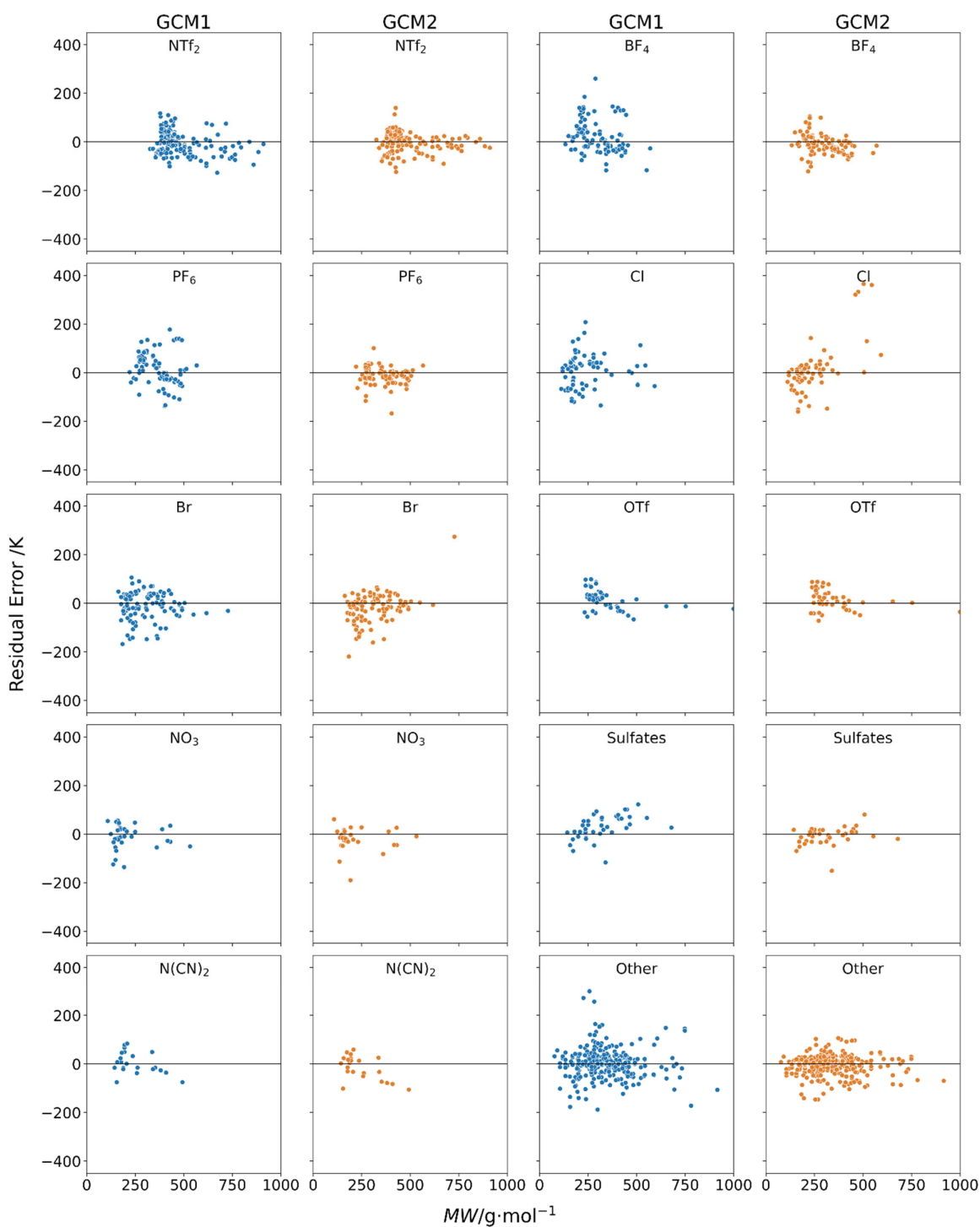
Figure 5. Individual residual plots of error versus molecular weight using GCM1 (blue) and GCM2 (orange) to estimate melting points for ILs containing several different anions.
