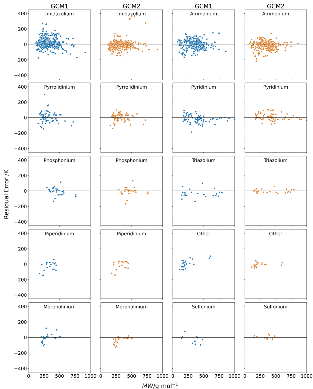
Figure 4. Individual residual plots of error versus molecular weight using GCM1 (blue) and GCM2 (orange) to estimate melting points for ILs containing several different cation types.
