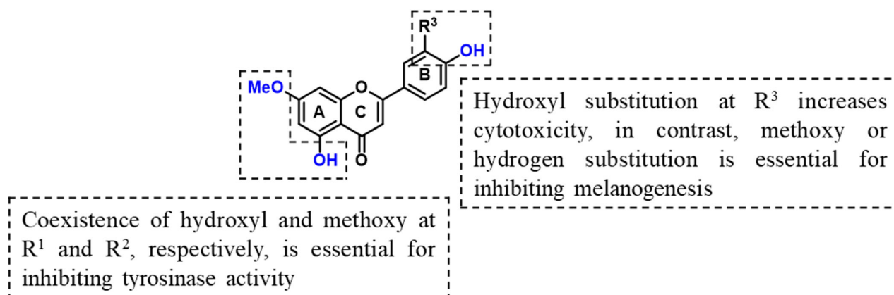
Figure 5. Velutin derivatives along with their structure–activity relationship for the inhibition of melanogenesis.
