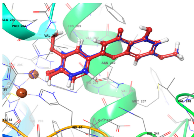
Figure 4. Molecular docking of tyrosinase binding with the V1 and V4 derivatives ( V1 : red sticks and V4 : blue sticks).
