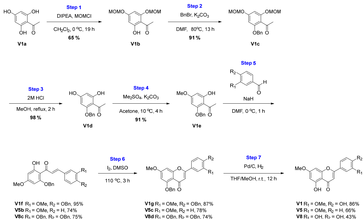
Scheme 1. Synthesis of V1 , V5 , and V8 derivatives.
