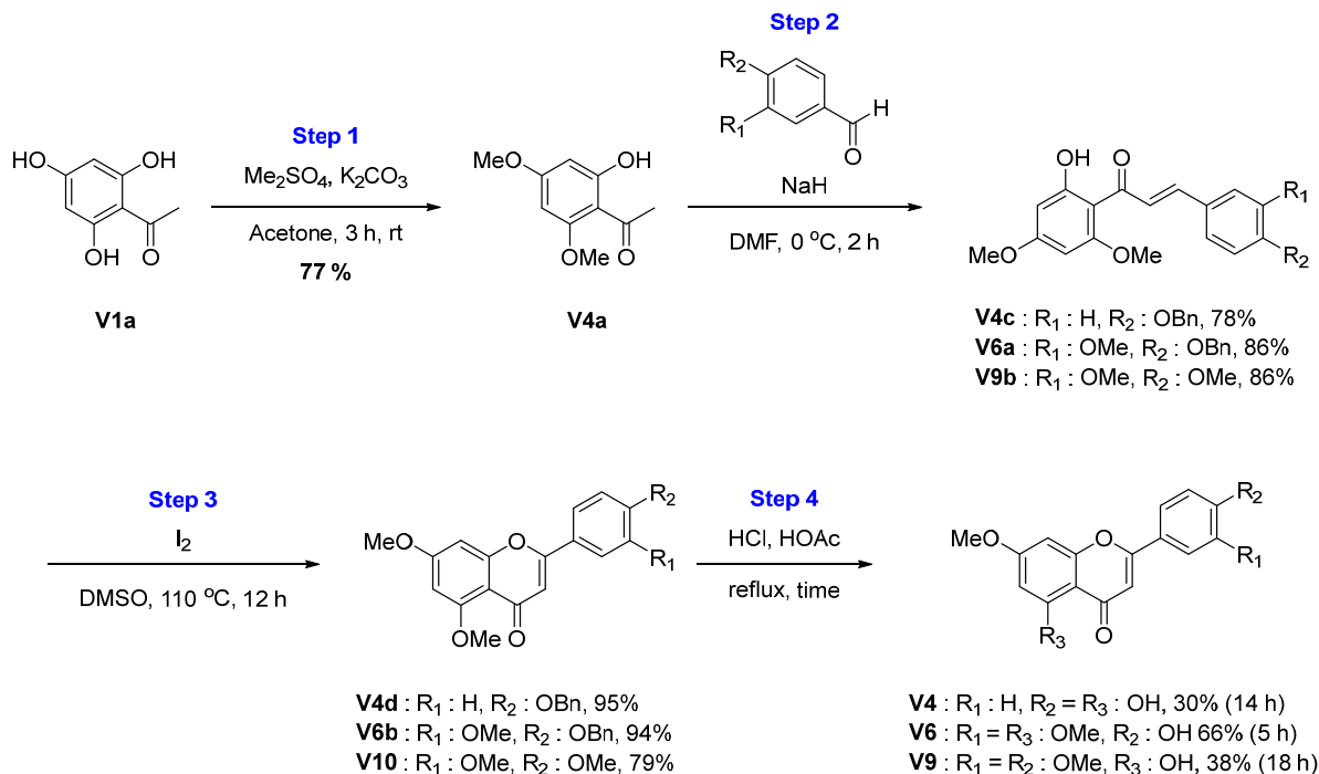
Scheme 3. Synthesis of V4 , V6 , V9 , and V10 derivatives.
