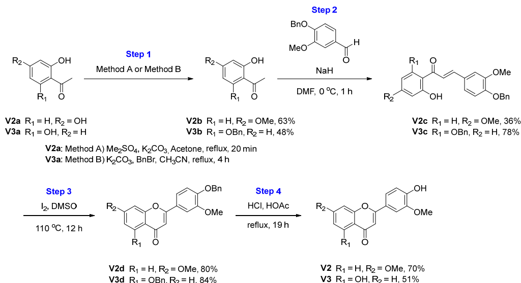
Scheme 2. Synthesis of V2 and V3 derivatives.
