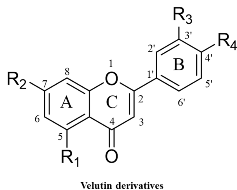
Figure 1. The chemical structure of flavones.
