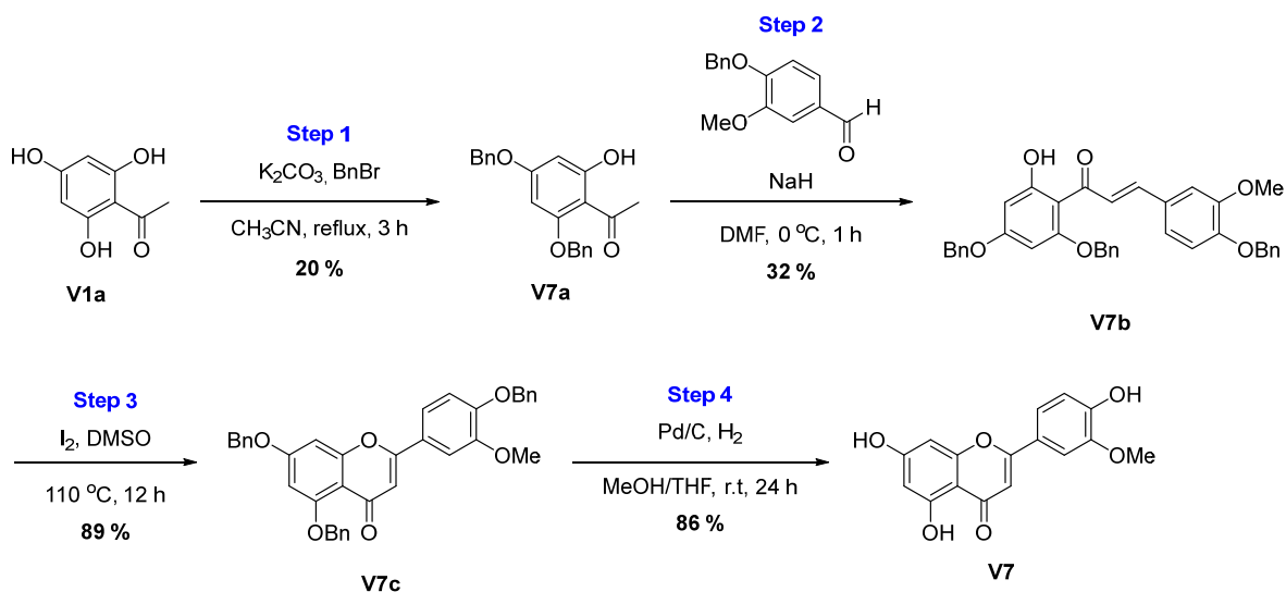
Scheme 4. Synthesis of V4 , V6 , V7 , V9 , and V10 derivatives.
