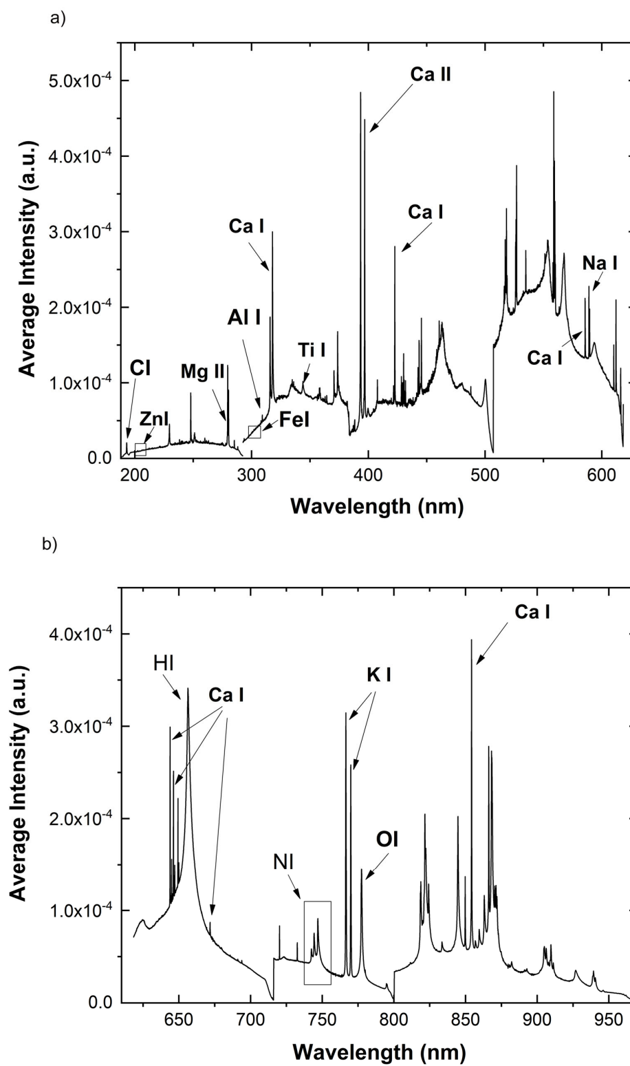
Figure 1. A typical LIBS spectrum of a sweet orange leaf in the spectral ranges 188.84–618.30 nm (a) and 618.30 nm–966.22 nm (b).
