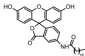
Figure 1. ODAF structure (lactone form).
