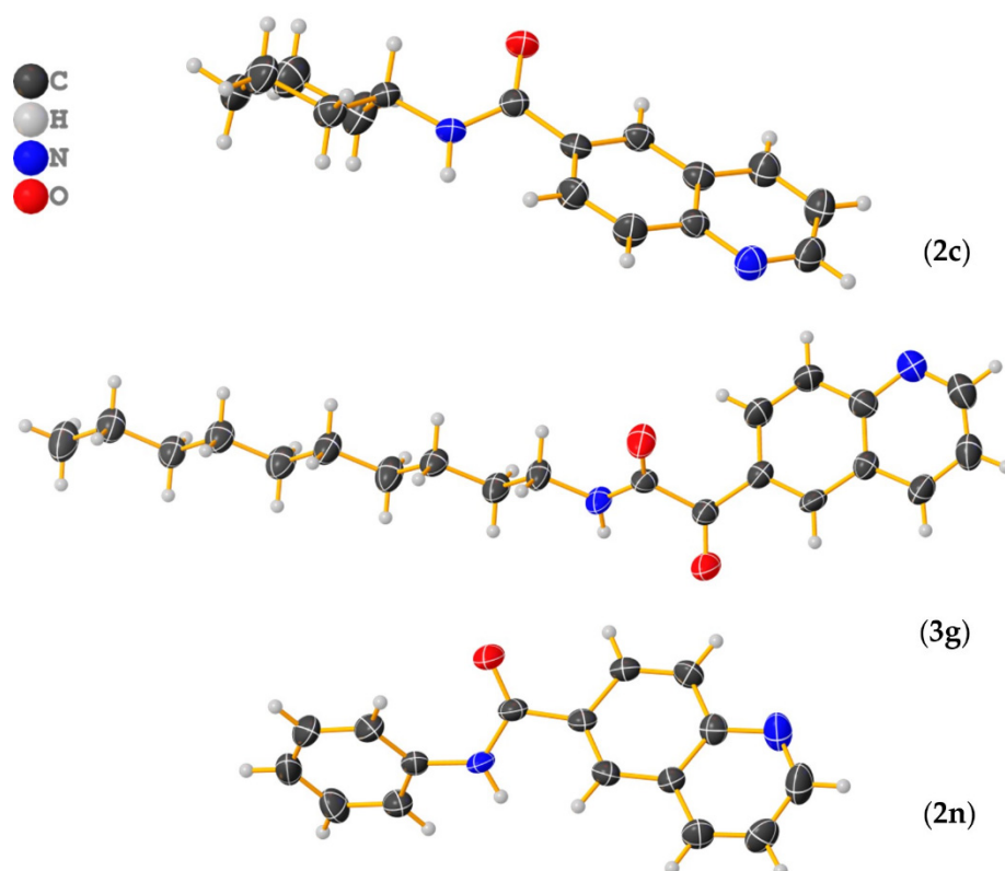
Figure 5. ORTEP style views of N -cyclohexylquinoline-6-carboxamide ( 2c ), N -decyl-2-oxo-2-(quinolin-6-yl)acetamide ( 3g ), and N -phenylquinoline-6-carboxamide ( 2n ), showing thermal displacement ellipsoids, drawn at the 50% probability level (Graphics were designed using Olex2 program.).
