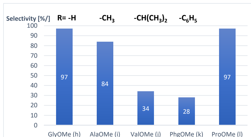
Figure 2. Influence of the side chains of amino acid methyl esters ( h–l ) on the selectivity towards the corresponding 2-ketocarboxamides in the aminocarbonylation of 6-iodoquinoline. (Reaction conditions: Pd(OAc) 2 /2 PPh 3 , 40 bar of CO, 50 °C, DMF, Et 3 N).
