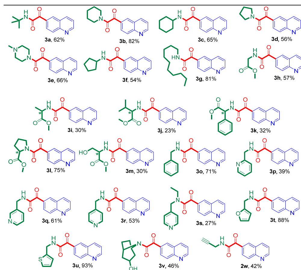
Figure 3. Nucleophile scope of aminocarbonylation: the quinoline-6-glyoxylamides synthesized in the aminocarbonylation of 1 at 40 bar CO pressure using a Pd(OAc) 2 /2 PPh 3 catalysts (further conditions are mentioned in the footnote of Table 2). (The yields of the isolated target compounds (%), based on the substrate ( 1 ), are indicated below the structure of the synthesized 2-ketocarboxamide derivatives.)
