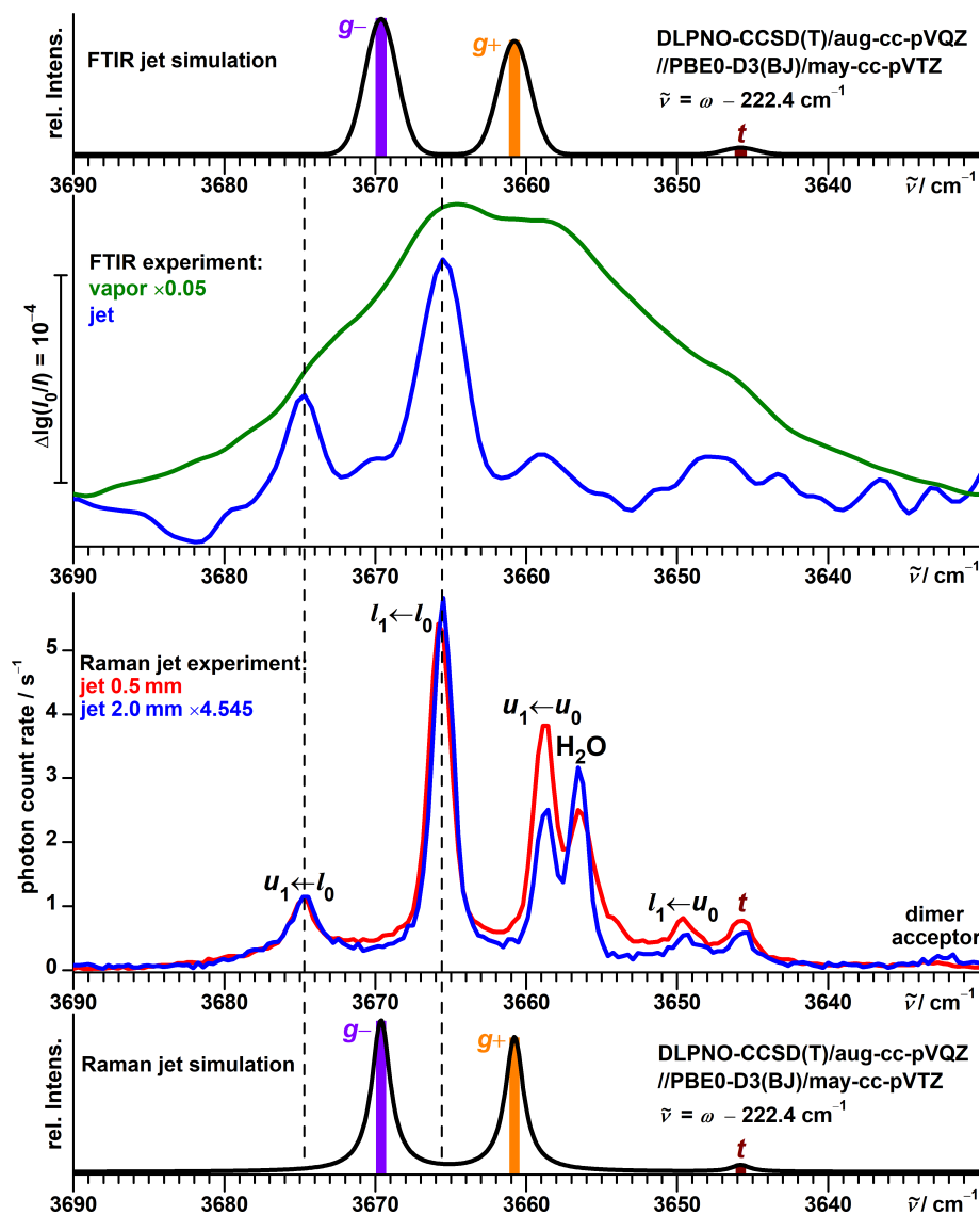
Figure 3. Top half: Comparison between simulated and experimental FTIR jet spectra of \alpha -fenchol. In addition, an FTIR spectrum of the vapor at ambient temperature is shown. Bottom half: Comparison between simulated and experimental Raman jet spectra of \alpha -fenchol at two different detection distances from the nozzle. For the simulations, a Boltzmann distribution of localized conformers is assumed at a conformational temperature of 100 K. Harmonic OH stretching wavenumbers are uniformly shifted according to the model of Ref. [51].
