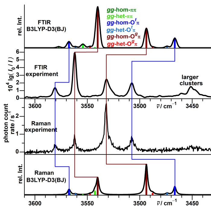
Figure 13. Comparison between experimental (inner) and simulated (outer) FTIR and Raman jet spectra for propargyl alcohol dimers. The simulations assume a conformational temperature of 100 K and identical vibrational and rotational partition functions except for the rotational symmetry number. In addition, the achirality (non-degeneracy) of gg\text{-het-}\pi\pi is considered in the statistical weight. Empirically applied are a Gaussian FWHM of 4.5\text{ cm}^{-1} for the FTIR simulation and a Lorentzian FWHM of 3\text{ cm}^{-1} for the Raman simulation. Harmonic OH stretching wavenumbers are shifted by -156\text{ cm}^{-1} as needed to match the g monomer spectral center of gravity.
