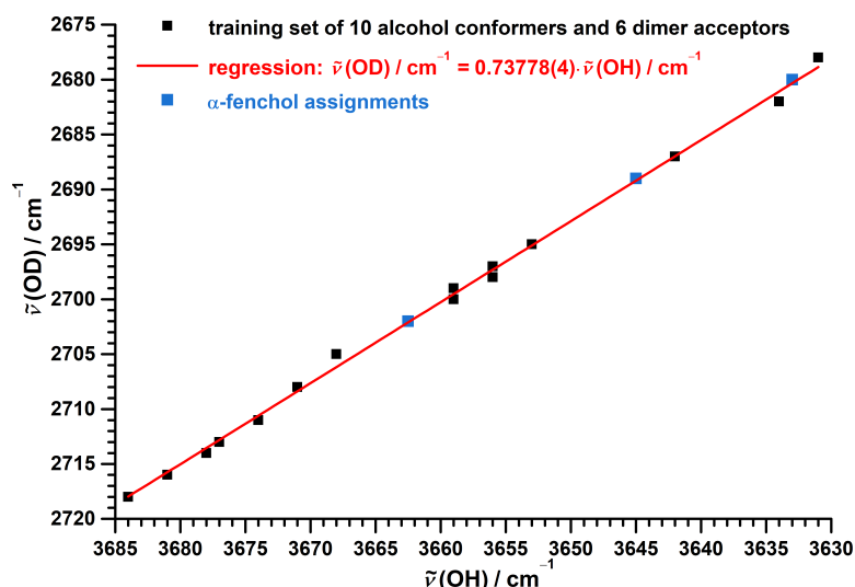
Figure 7. Correlation between experimental jet OD and OH stretching fundamental wavenumbers of alcohol monomers and alcohol dimer acceptors. Used data [75–77,92] for the training set are listed in Table S3. The linear regression for the training set uses a fixed intercept of zero.
