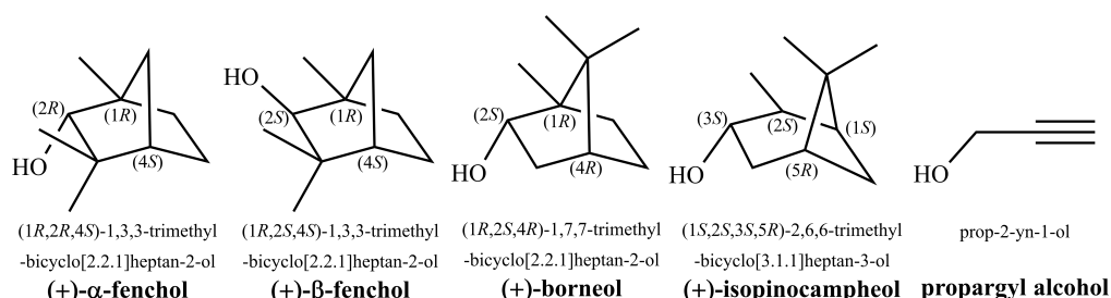
Figure 1. Structural formulas, systematic names and used trivial names of alcohols discussed in this study.
