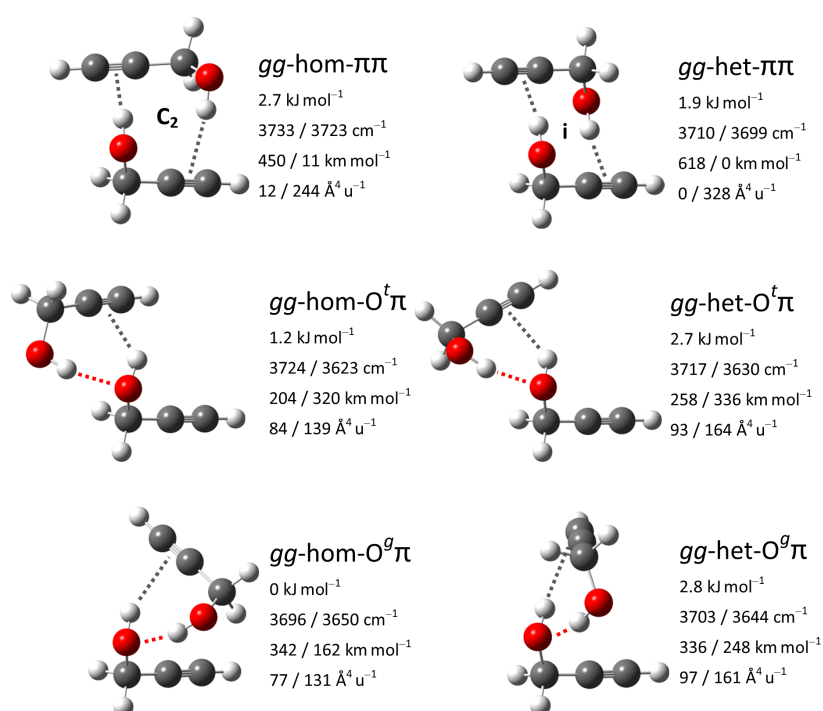
Figure 12. Leading propargyl alcohol dimer structures with harmonically zero-point-corrected relative energies, unscaled harmonic OH stretching wavenumbers as well as associated IR intensities and Raman activities at B3LYP-D3(BJ)/may-cc-pVTZ level. Indicated, where present, are symmetry elements as well as OH \cdots O hydrogen bonds by red and OH \cdots \pi by gray dotted lines.
