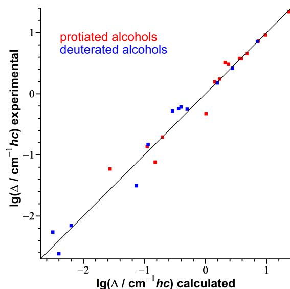
Figure 9. Correlation between logarithmized experimental tunneling splittings [20,87,94–110] and calculated ones with the 1D torsion code based on electronic B3LYP-D3(BJ)/may-cc-pVTZ potentials for 27 isotopologs of 16 symmetric alcohols. The diagonal line represents perfect agreement. Data points are given in Table S5, diagrams with torsional potentials, energy levels, probability distributions and moment of inertia for all species are available in Figures S9–S25.
