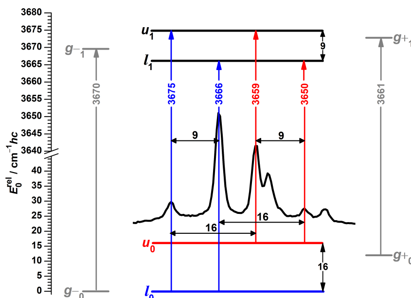
Figure 4. Raman spectral pattern in the OH stretching spectrum of \alpha -fenchol with repeating separations (black horizontal double-headed arrows) translated into torsional splittings (black vertical double-headed arrows). The ground state l_0 and transitions originating from it are colored blue, for the first excited torsional state u_0 likewise red, for hypothetical localized g^- and g^+ states gray, the latter based on DLPNO-CCSD(T)/aug-cc-pVQZ//PBE0-D3(BJ)/may-cc-pVTZ calculations with shifted harmonic OH stretching wavenumbers [51]. l stands for lower and u for upper torsional state, the index 0 or 1 indicates the OH stretch quantum number.
