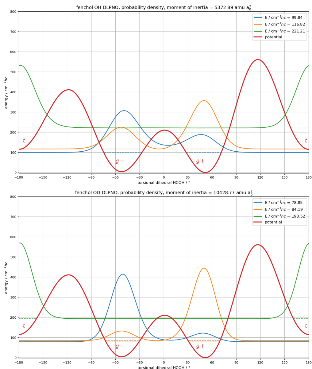
Figure 10. Electronic torsional potential (red trace) of (+)- \alpha -fenchol calculated at B3LYP-D3(BJ)/may-cc-pVTZ level and scaled to DLPNO-CCSD(T)/aug-cc-pVQZ single-point corrections for the six stationary points. A constant moment of inertia, as calculated for the g^- minimum geometry, was used. For the protiated (top) and the deuterated alcohol (bottom), the two lowest torsional states (blue and orange horizontal dashed traces) are separated by 17.0 (OH) and 5.3 \text{cm}^{-1}hc (OD) and their probability densities (blue and orange solid traces) are strongly (OH: 69%/31%) to moderately (OD: 88%/12%) delocalized between the g^-/g^+ potential wells. In contrast, for the third torsional state, the probability density (green solid trace) is very strongly (>99%) in the t potential well.
