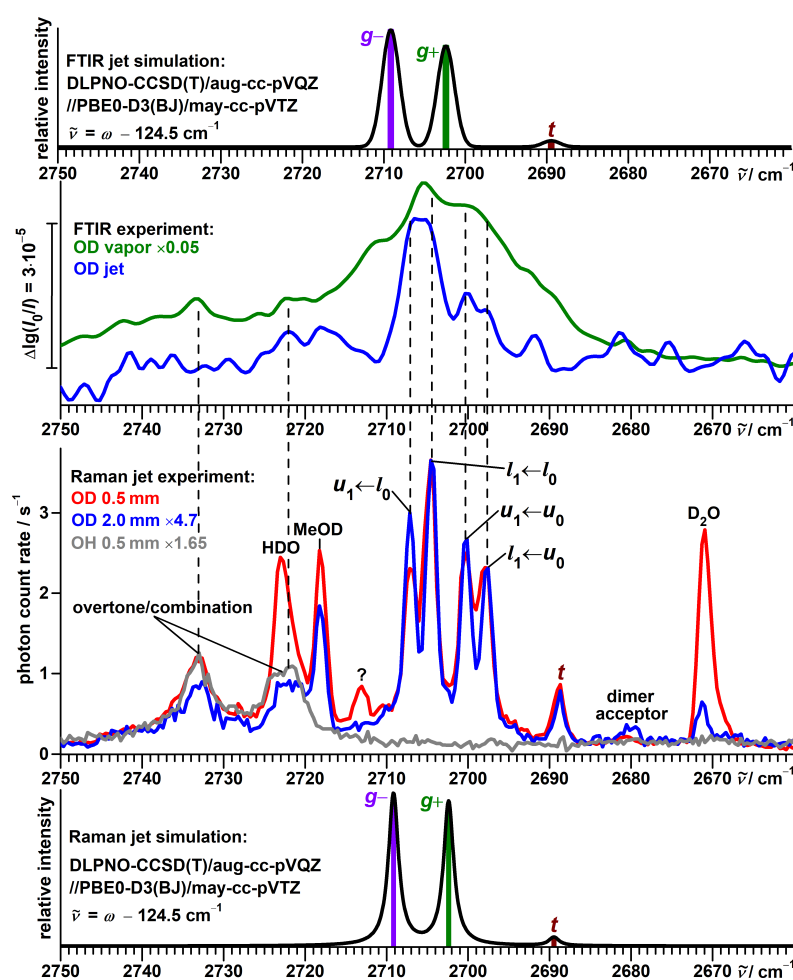
Figure 5. Top half: Comparison between simulated and experimental FTIR jet spectra of \alpha -fenchol-OD. In addition, an FTIR spectrum of the vapor at ambient temperature is shown. Bottom half: Comparison between simulated and experimental Raman jet spectra of \alpha -fenchol-OD at two different detection distances from the nozzle in the OD stretching region. In addition, a spectrum of \alpha -fenchol-OH in this spectral region is shown. For the simulations, a Boltzmann distribution of localized conformers is assumed at a conformational temperature of 100 K. Harmonic OD stretching wavenumbers are uniformly shifted according to the model of Ref. [51].
