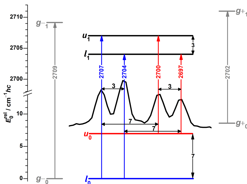
Figure 6. Raman spectral pattern in the OD stretching spectrum of \alpha -fenchol with repeating separations (black horizontal double-headed arrows) translated into torsional splittings (black vertical double-headed arrows). The ground state l_0 and transitions originating from it are colored blue, for the first excited torsional state u_0 likewise red, for hypothetical localized g^- and g^+ states gray, the latter based on DLPNO-CCSD(T)/aug-cc-pVQZ//PBE0-D3(BJ)/may-cc-pVTZ calculations with shifted harmonic OD stretching wavenumbers [51]. l stands for lower and u for torsional upper state, the index 0 or 1 indicates the OD stretch quantum number.
