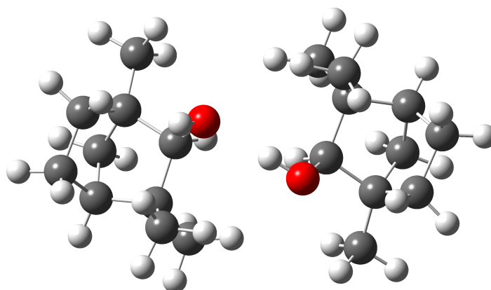
Figure 15. Most stable dimer of (+)- \alpha -fenchol at B3LYP/may-cc-pVTZ level viewed along the approximate C_2 symmetry axis.
