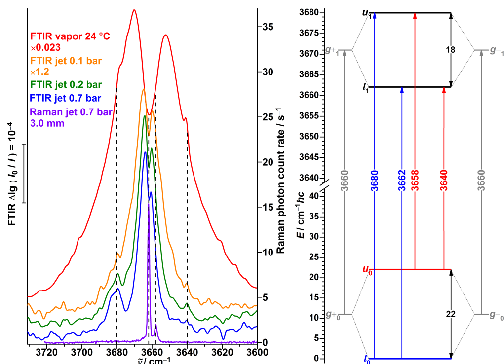
Figure 11. Left: FTIR jet and vapor spectra as well a Raman spectrum of propargyl alcohol in the OH stretching monomer spectral region. Assigned positions of band centers are indicated with dashed lines. Right: Energy level scheme with the ground state and transitions originating from it in blue, likewise for the upper tunneling state in red, as well as for hypothetical localized states in gray.
