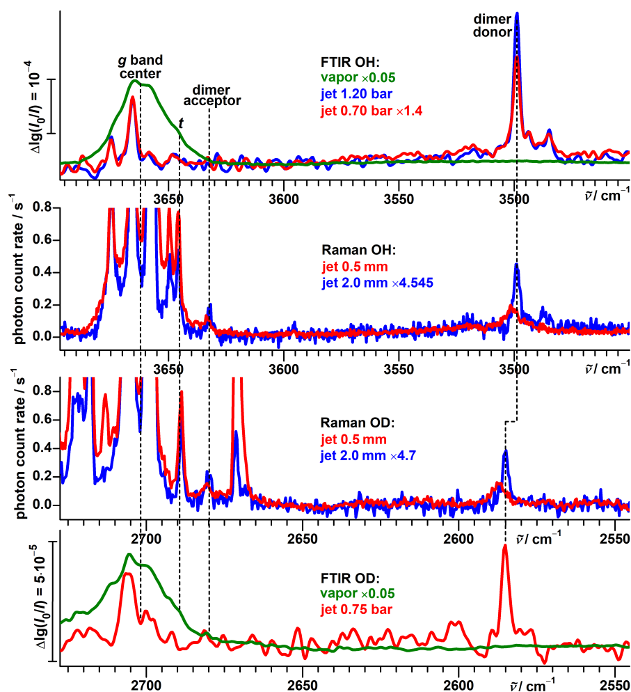
Figure 14. Comparison between FTIR and Raman spectra of protiated (top traces) and deuterated (bottom traces) (+)- \alpha -fenchol. The wavenumber axes for the OH and OD stretching regions are aligned according to 0.73778 \cdot \tilde{\nu}(\text{OH}) = \tilde{\nu}(\text{OD}) .
