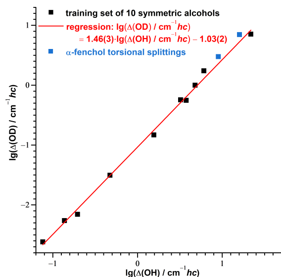
Figure 8. Correlation between the logarithmized experimental tunneling splittings \lg(\Delta/\text{cm}^{-1}hc) of deuterated and protiated symmetric alcohols (Direct Correlation Model of Ref. [93], details given there) compared with the torsional splittings assigned for the ground and the OH/OD stretch excited state of \alpha -fenchol.
