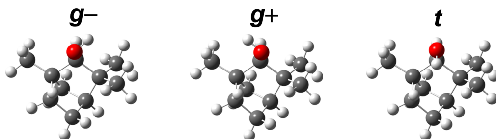
Figure 2. Optimized torsional conformers of (+)- \alpha -fenchol at B3LYP-D3(BJ)/may-cc-pVTZ level. They are labeled according to the qualitative arrangement of the \text{HOC}_{\alpha}\text{H} dihedral: gauche ( g ) \approx -60^{\circ} or +60^{\circ} , or trans ( t ) \approx \pm 180^{\circ} .
