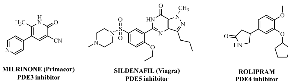
Figure 1. PDEs inhibitors.
