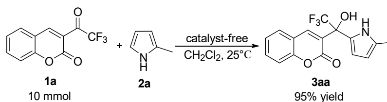
Scheme 1. Scaled-up experiment of the one-pot reaction.
