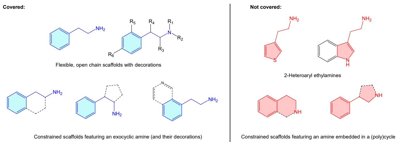
Figure 2. Description of 2-phenethylamine scope of the present review.
