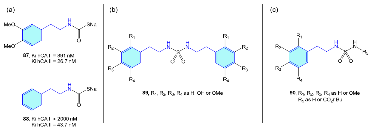
Figure 8. 2-Phenylethyl-based CA ligands.
