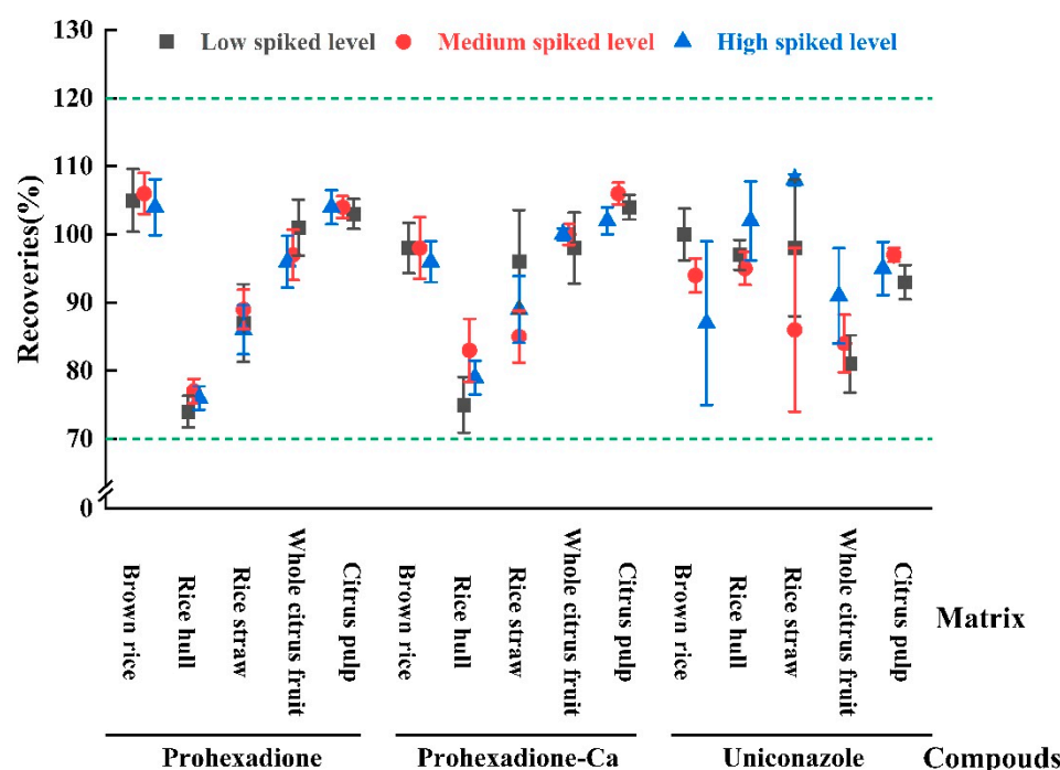
Figure 2. Recoveries of prohexadione, prohexadione-Ca and uniconazole in rice and citrus.
