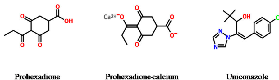
Figure 1. Chemical structure of plant growth regulators (prohexadione, prohexadione-Ca, and uniconazole).
