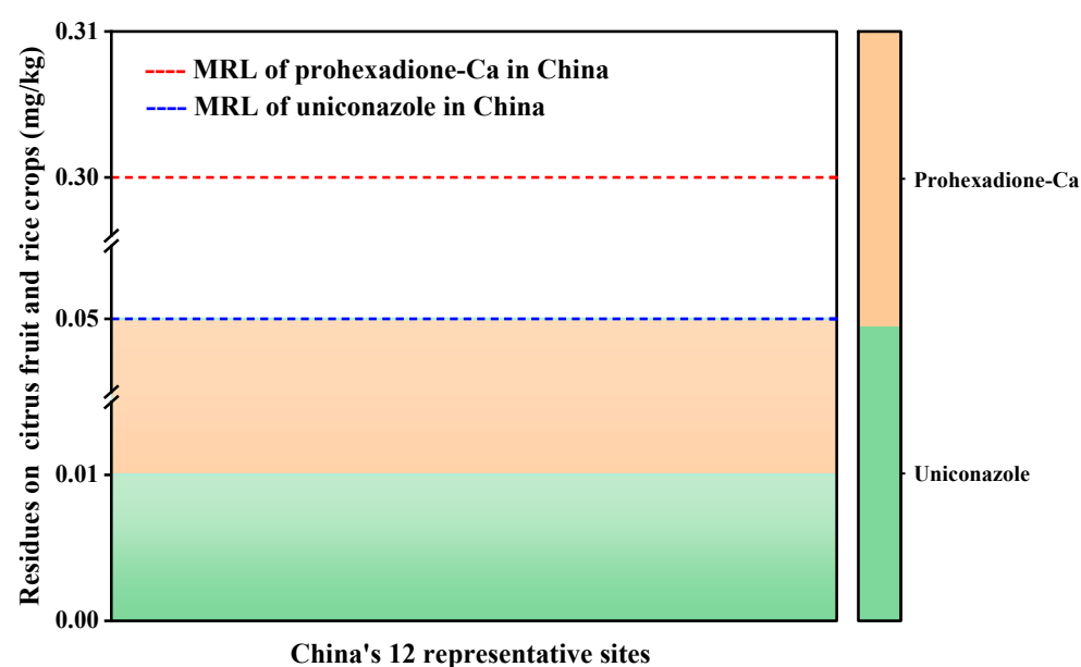
Figure 3. Residues and MRLs of prohexadione-Ca and uniconazole at 12 representative sites.
