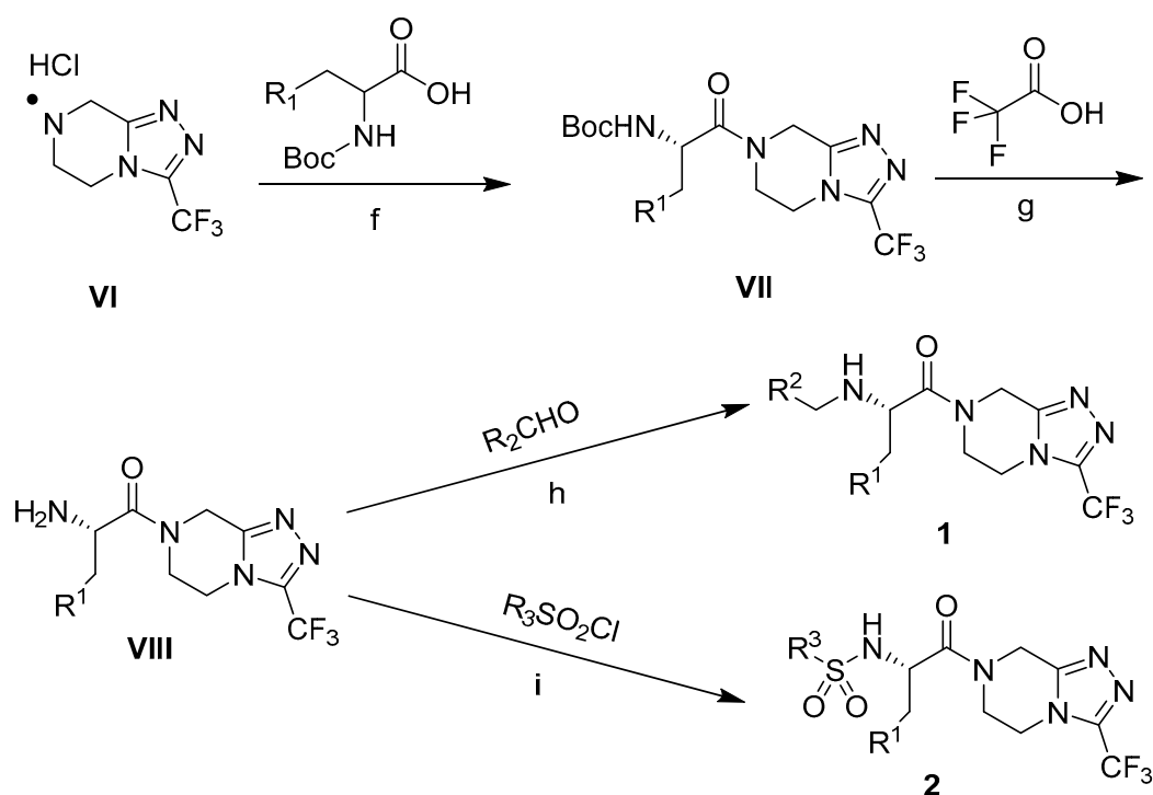
Scheme 2. Synthesis of triazolo[4,3- a ]pyrazine derivatives. Reagents and conditions: (f) DCC, Et 3 N, DCM, 0 °C to r.t., 36 h; (g) DCM, r.t., 4 h; (h) NaBH 3 CN, CH 3 COOH, MeOH, 0 °C to r.t., overnight; (i) Et 3 N, DCM, 0 °C to r.t., 3 h.
