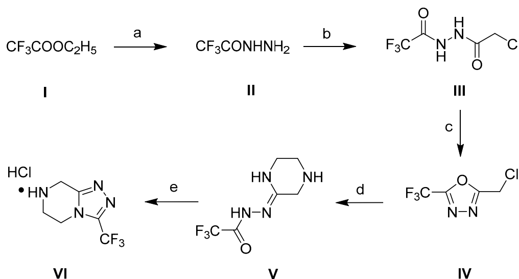
Scheme 1. Synthesis of 3-(trifluoromethyl)-1,2,4-triazolo[4,3- a ]pyrazine as the key scaffold. Reagents and conditions: (a) 35% NH 2 NH 2 ·H 2 O, CH 3 CN, 20 °C, 1 h; (b) NaOH (50%), ClCH 2 COCl, CH 3 CN, 10 °C, 3 h; (c) POCl 3 , CH 3 CN, 80 °C, 24 h; (d) 3 equiv. of H 2 NCH 2 CH 2 NH 2 , MeOH, −20 °C, 1 h; (e) Con. HCl, MeOH, 55 °C, 1 h.
