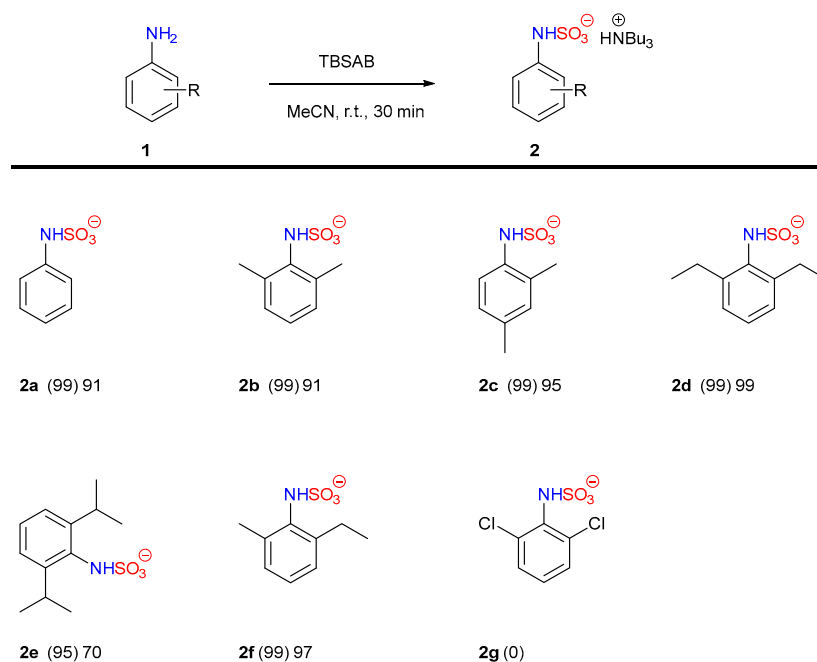
Scheme 3. Synthesis of N (sp 2 )-anilino sulfamates using TBSAB. The tributylammonium cation is omitted for clarity. Key: percentage conversion as measured by 1 H NMR spectroscopy is reported in parentheses, and isolated yield thereafter.
