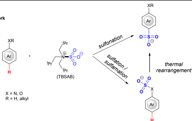
Scheme 1. Previous Approaches (a–c) towards the synthesis of p -aminobenzene sulfonic acid compounds using an N - to C-SO 3 transfer and this study: TBSAB is used to introduce the SO 3 group into aromatic systems. The tetrabutylammonium cation is omitted for clarity [16–20].
