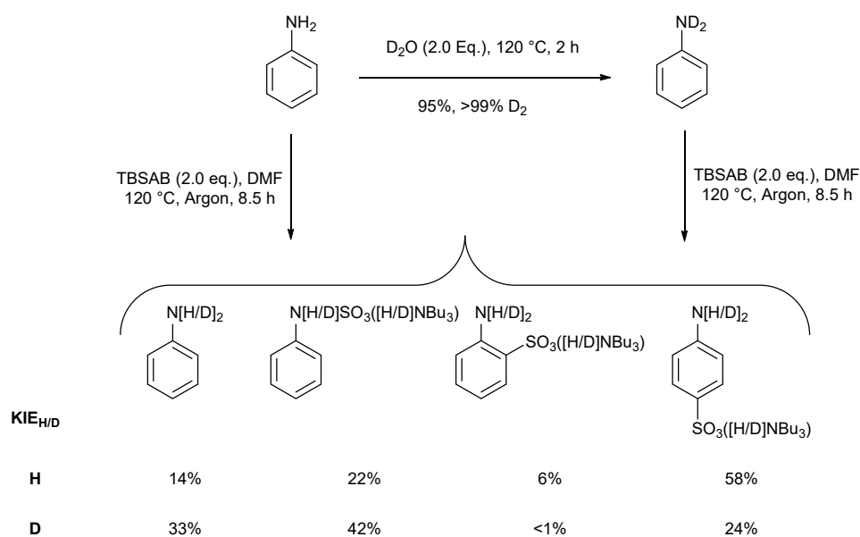
Scheme 7. \text{KIE}_{\text{H}/\text{D}} effects on aniline sulfamation/sulfonation. Percentage conversion measured by ^1\text{H} NMR spectroscopic analysis.
