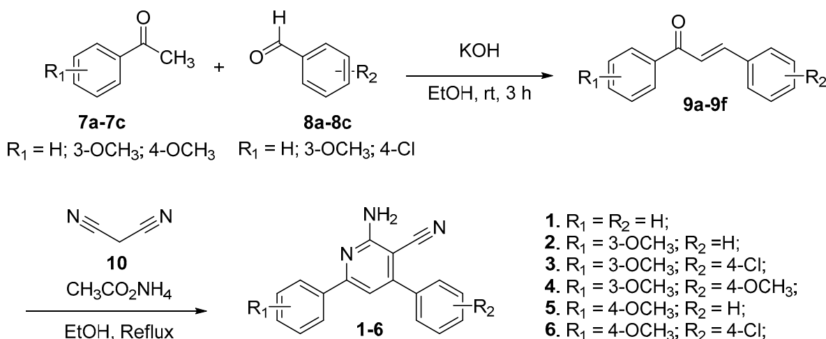
Scheme 1. Synthesis of APNs ( 1–6 ).
