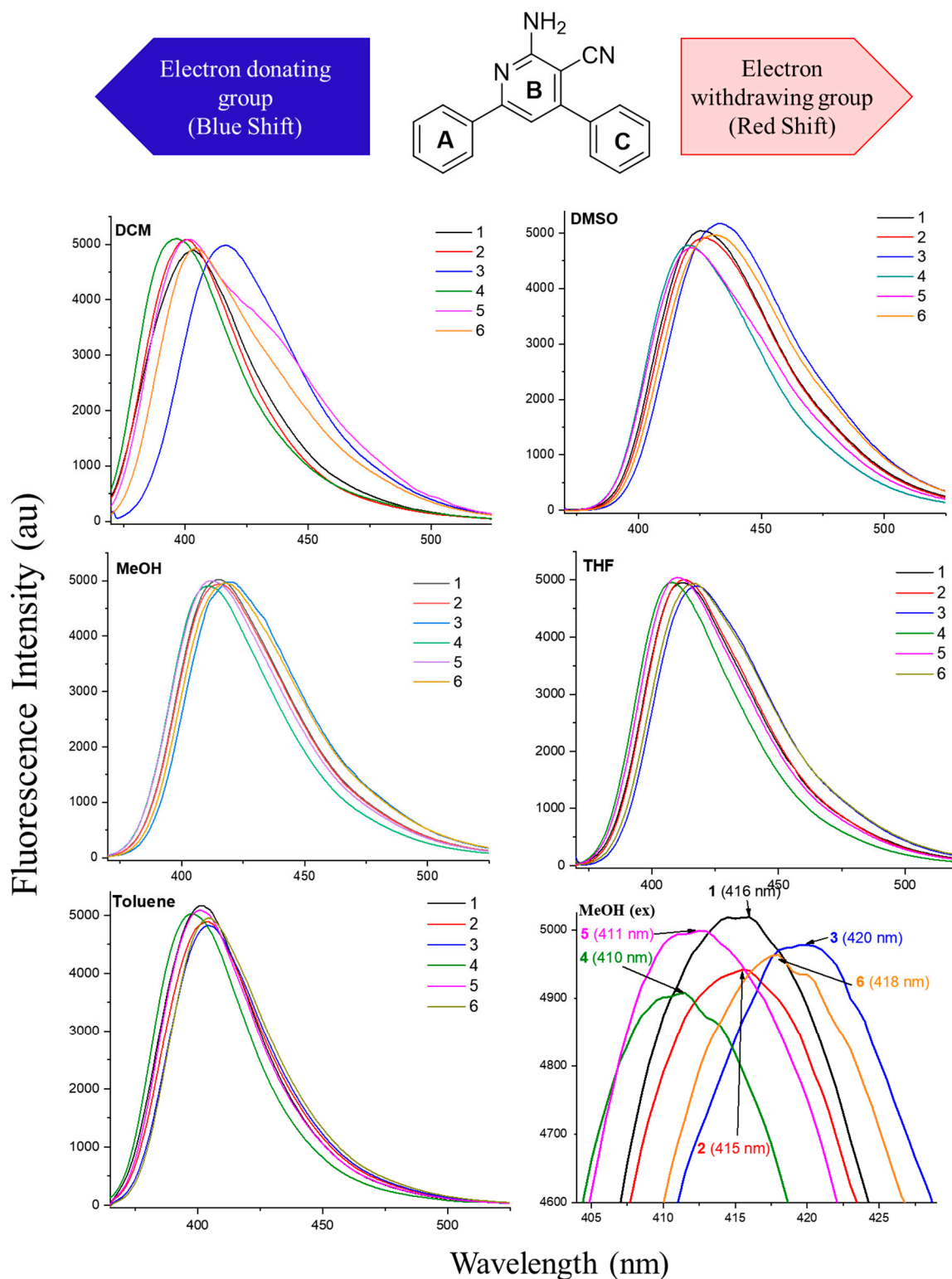
Figure 3. Electro-withdrawing/donating effect of fluorescence emission of compounds 1–6.
