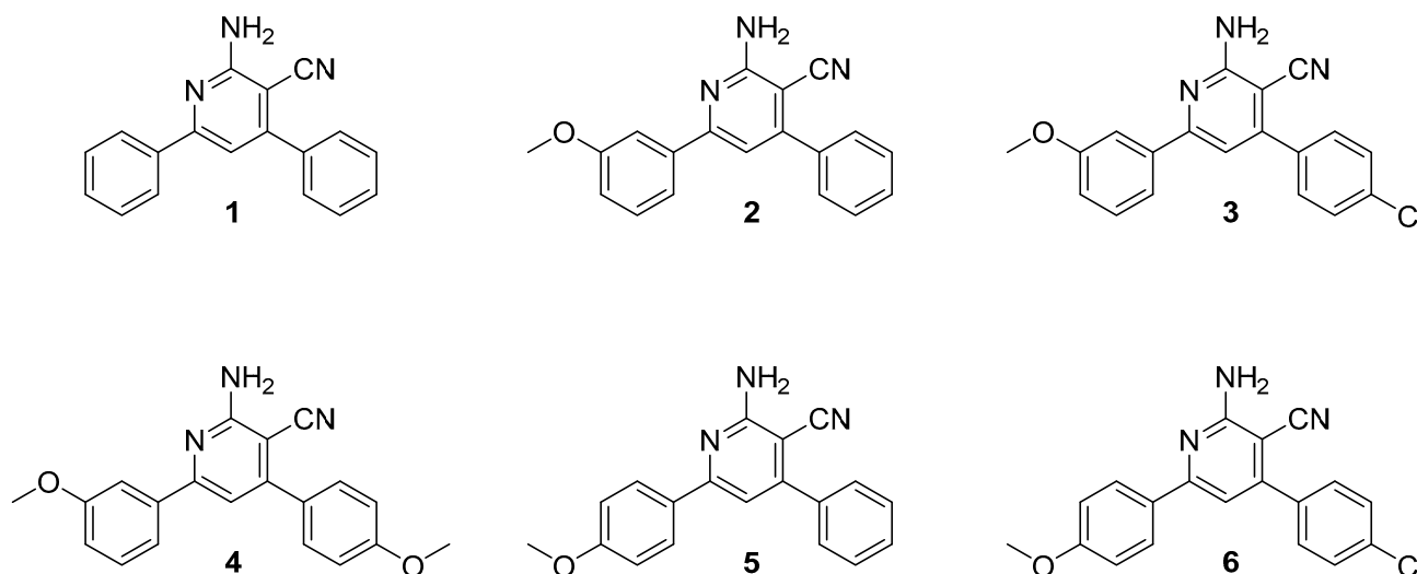
Figure 1. 2-Amino-4,6-diphenylnicotinonitrile derivatives (1–6).
