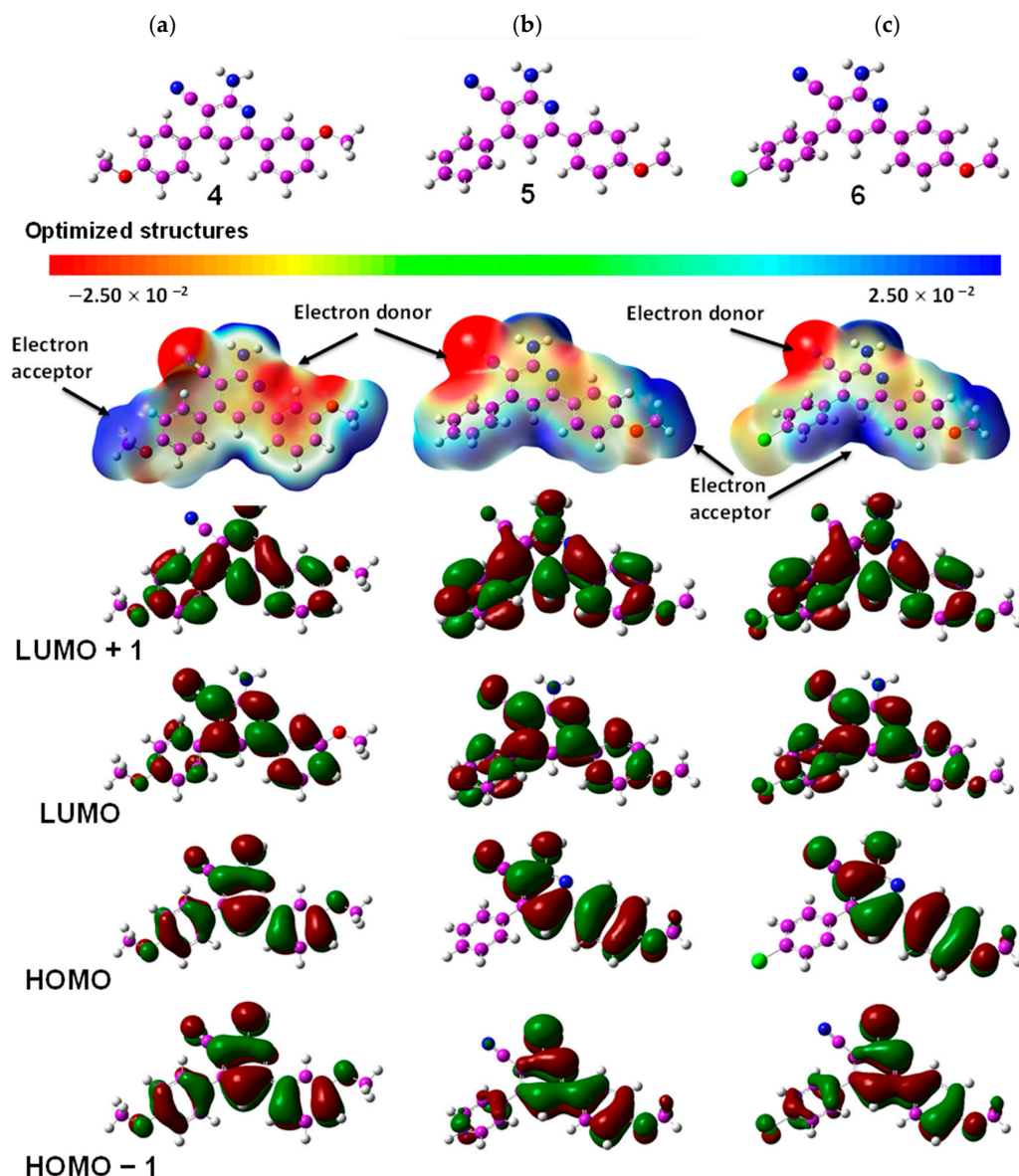
Figure 5. Optimized gas-phase molecular structures, ESP, LUMO, and HOMO structures of APNs 4–6: ((a) compound 4; (b) compound 5; and (c) compound 6) at the B3LYP/6-311++g(d,p) level of theory in the water solvent system (color code: carbon: purple; hydrogen: white; nitrogen: blue; oxygen: red; sulfur: yellow). The order of increasing ESP (i.e., highest negative value) is red > orange > yellow > green > blue (indicated by the arrows).
