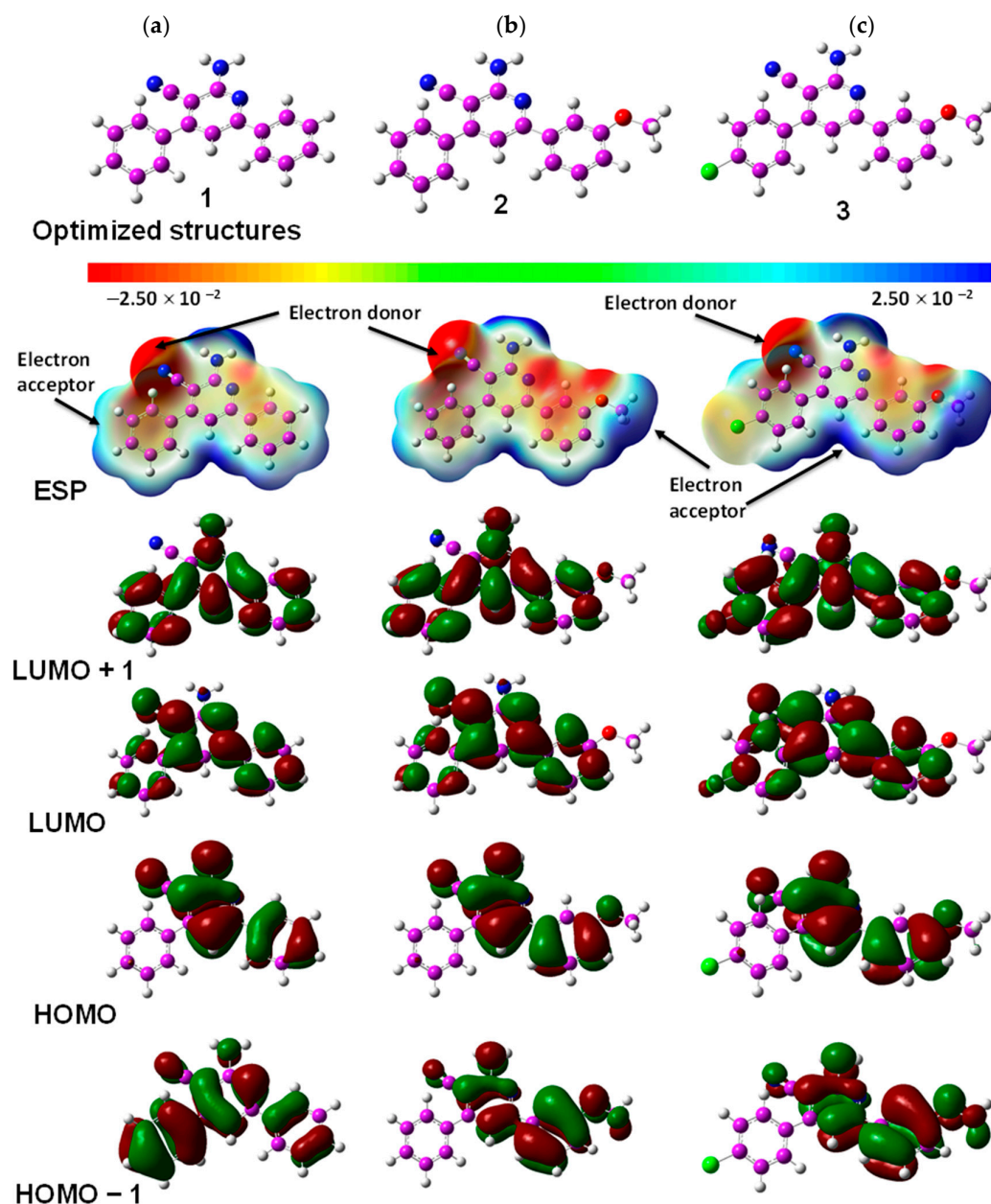
Figure 4. Optimized gas-phase molecular structures, ESP, LUMO, and HOMO structures of APNs 1–3 ((a) compound 1; (b) compound 2; and (c) compound 3) at the B3LYP/6-311++g(d,p) level of theory in the water solvent system (color code: carbon: purple; hydrogen: white; nitrogen: blue; oxygen: red; sulfur: yellow). The order of increasing ESP (i.e., highest negative value) is red > orange > yellow > green > blue (indicated by the arrows).
