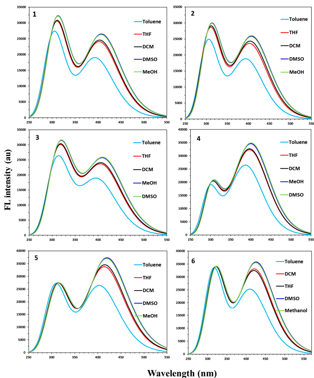
Figure 6. TD-DFT-calculated electronic fluorescence emission spectra of synthesized APNs (1–6) at the TD-DFT/B3LYP/6-311++g(d,p) basis set level of theory in toluene, THF, DCM, DMSO, and methanol solvent systems.
