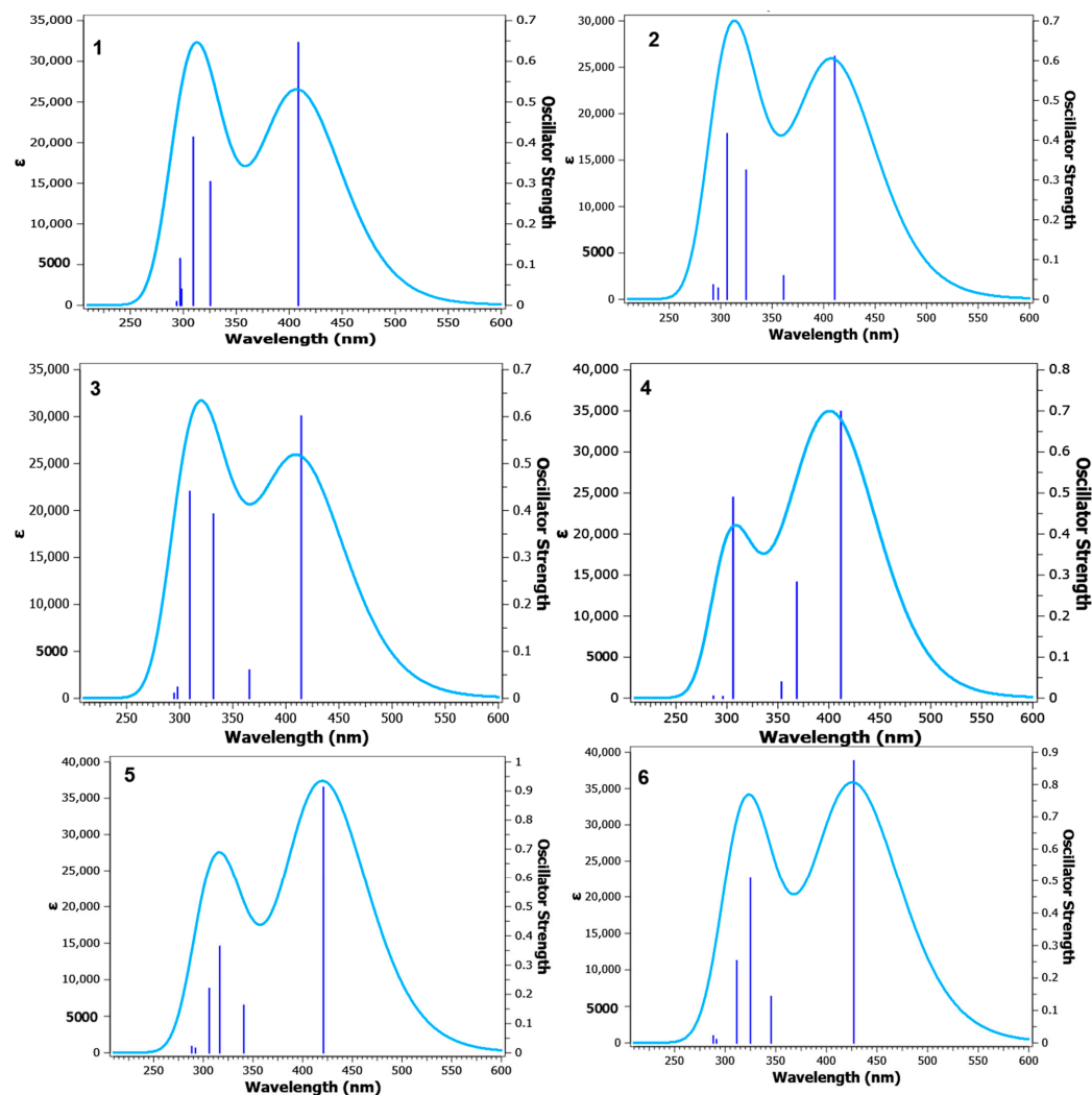
Figure 9. TD-DFT-calculated electronic fluorescence emission spectra of compounds 1–6 at the TD-DFT/B3LYP/6-311++g(d,p) basis set level of theory in a DMSO solvent system.
