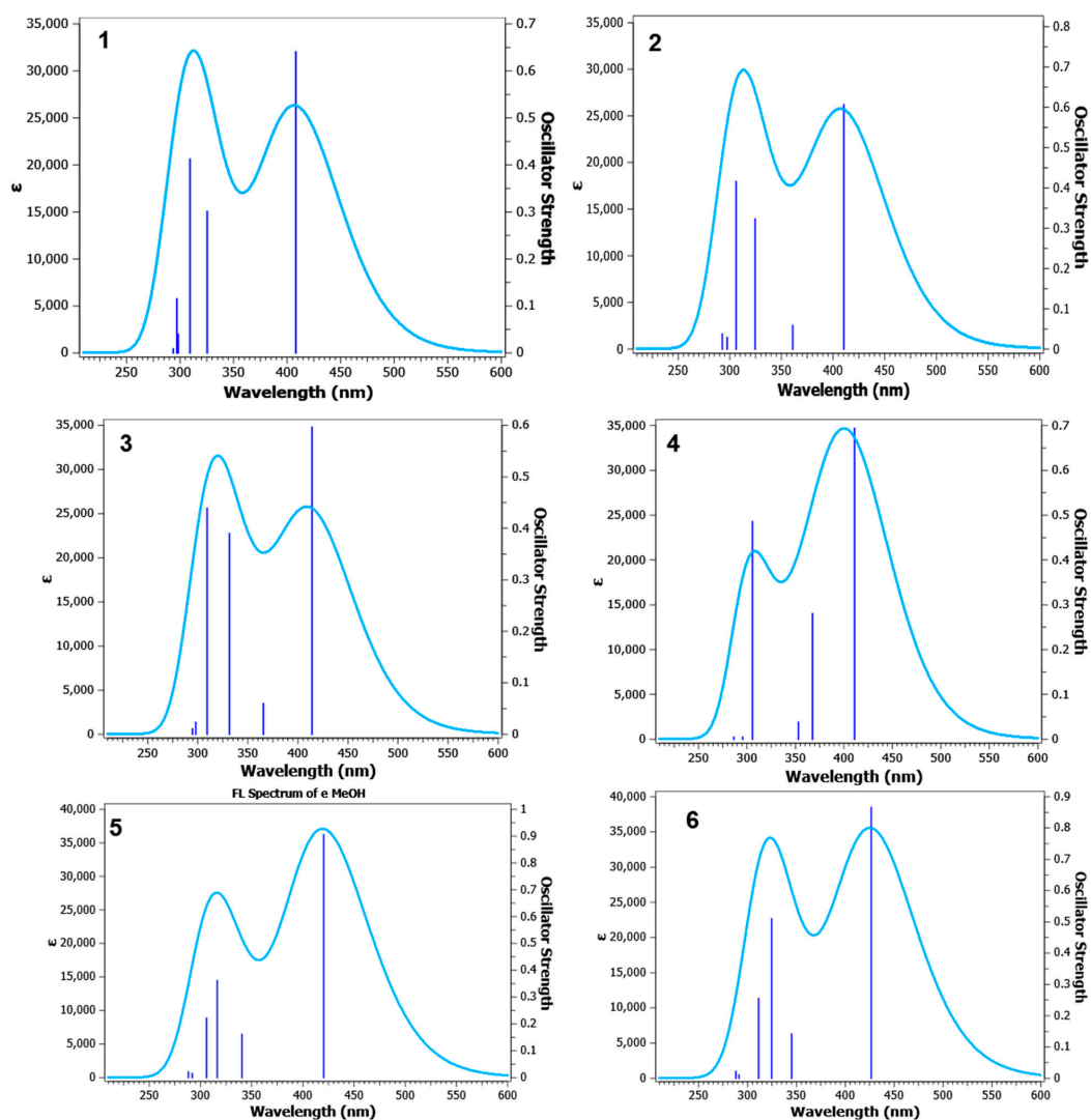
Figure 8. TD-DFT-calculated electronic fluorescence emission spectra of compounds 1–6 at the TD-DFT/B3LYP/6-311++g(d,p) basis set level of theory in a methanol solvent system.
