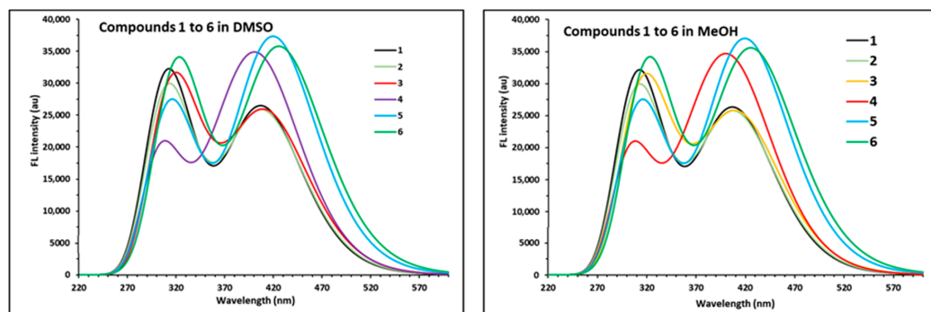
Figure 7. Comparison of the TD-DFT-calculated electronic fluorescence emission spectra of compounds 1–6 at the TD-DFT/B3LYP/6-311++g(d,p) basis set level of theory in DMSO and methanol solvent systems.
