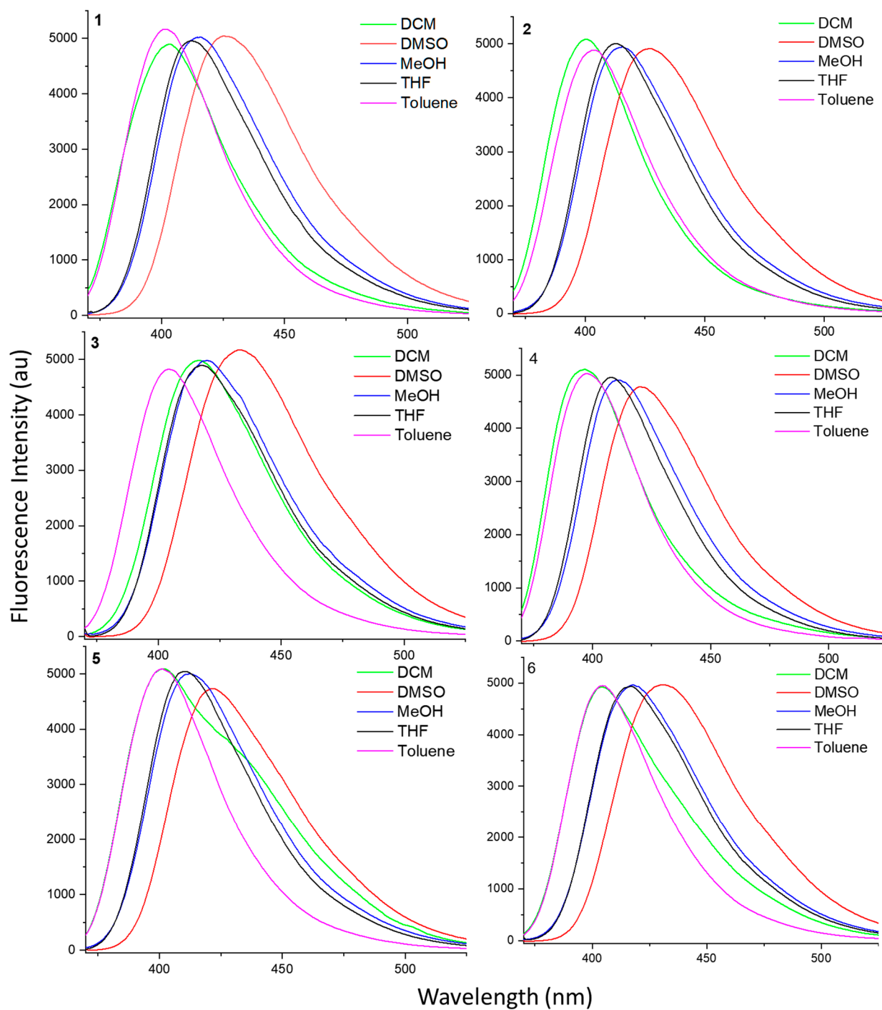
Figure 2. Fluorescence (emission) spectra of synthesized compounds 1–6 in different solvents at 1.45 \times 10^{-8} M.
