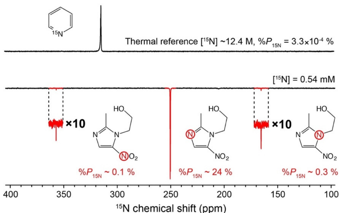
Figure 1. Example of hyperpolarization. (Top) A typical ^{15}\text{N} NMR spectrum of ^{15}\text{N} -pyridine (~99% ^{15}\text{N} labeling) recorded at 9.4 tesla. (Bottom) SABRE-enhanced ^{15}\text{N} NMR spectrum of metronidazole at 150 mM ( ^{15}\text{N} nuclei at natural isotopic abundance of 0.35%) after 30 s of parahydrogen bubbling (50% p\text{H}_2 enrichment fraction). Nitrogen-15 in the -\text{NO}_2 group is demonstrated to have a T_1 of ~15 min. Reproduced with permission from [13].
