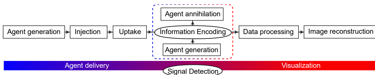
Figure 3. Stages of molecular imaging using exogenous and endogenous (dashed line) contrast agents.
