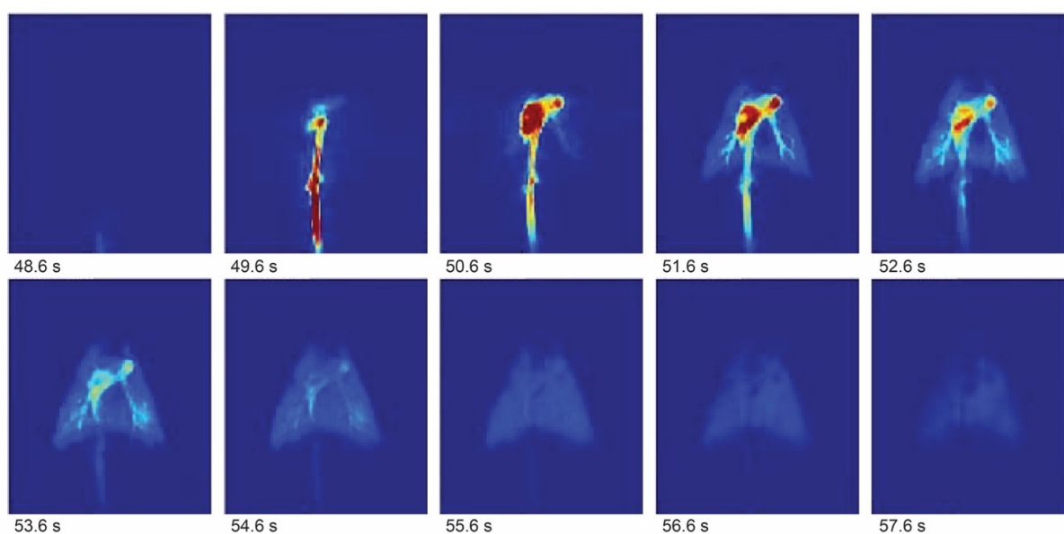
Figure 2. Hyperpolarization-enhanced ^{13}\text{C} magnetic resonance images showing the lungs of a pig after injection of hyperpolarized ^{13}\text{C} -2-hydroxyethylacrylate with 1 s time resolution. Adapted with permission from [47].
