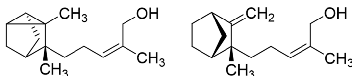
Figure 1. Structures of (Z)- \alpha -santalol (left) and (Z)- \beta -santalol (right).
