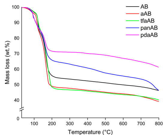
Figure 2. Thermograms of AB, aAB, tfaAB, panAB, and pdaAB, collected using heating rate of 10\text{ }^{\circ}C/min .
