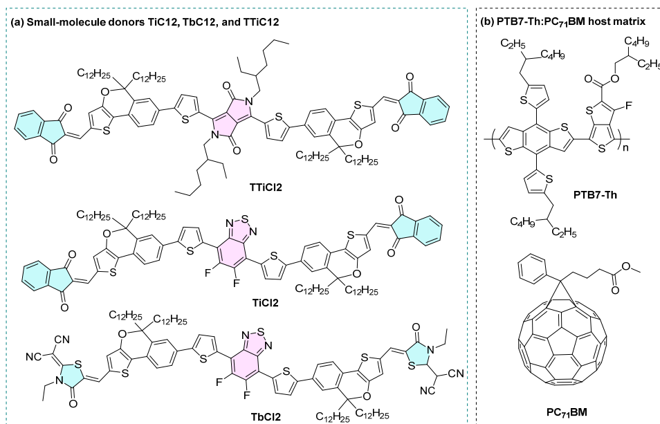
Figure 1. Molecular structure formula of the organic materials (a) TTiC12, TiC12, TbC12, (b) PTB7-Th and PC 71 BM.
