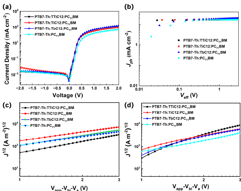
Figure 4. (a) Dark current; (b) the corresponding J_{ph} - V_{eff} curve; (c) the hole mobility of devices based on PTB7-Th:PC 71 BM system and (d) the corresponding electron mobility.
