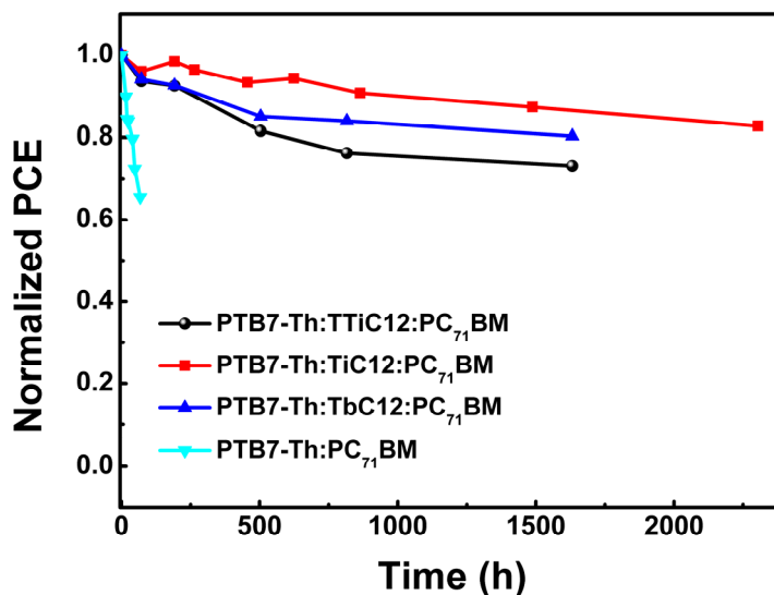
Figure 6. Time stability of devices in PTB7-Th:PC 71 BM system under nitrogen environment.
