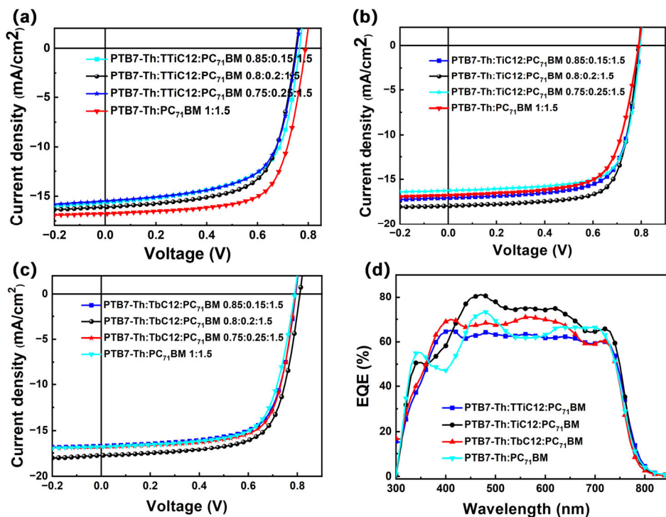
Figure 3. J - V curves of (a) PTB7-Th:TTiC12:PC 71 BM, (b) PTB7-Th:TiC12:PC 71 BM, (c) PTB7-Th:TbC12:PC 71 BM devices of different proportions and (d) EQE curves of the optimal binary and ternary OSCs.
