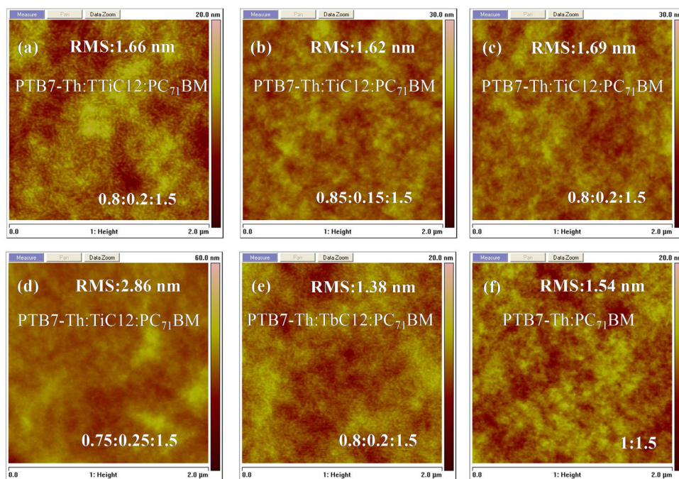
Figure 5. AFM morphology of (a) PTB7-Th:TTiC12:PC 71 BM, (b–d) PTB7-Th:TiC12:PC 71 BM, (e) PTB7-Th:TbC12:PC 71 BM and (f) PTB7-Th:PC 71 BM blend films with different proportions.
