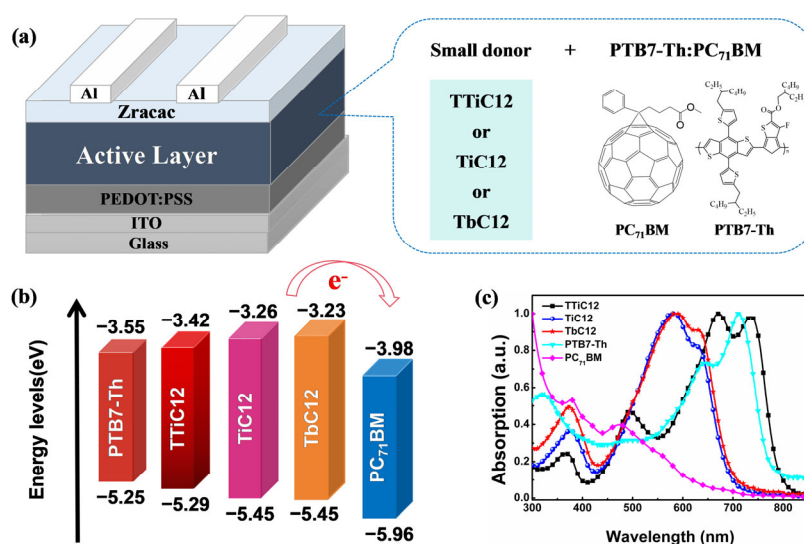
Figure 2. (a) Device structure diagram, (b) energy-level diagram, (c) UV-vis absorption spectrum.
