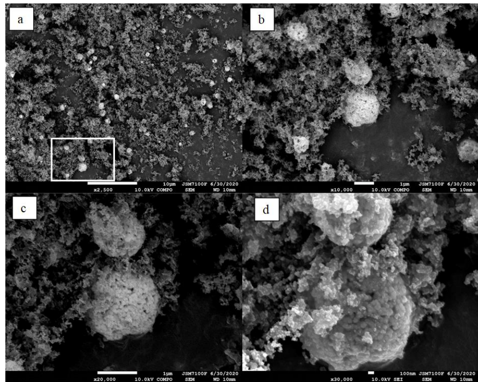
Figure 2. (a–d) Examples of SEM images of MOC10 nanocomposites. Scale bar sizes: (a) 10 \mu\text{m} , (b) 1 \mu\text{m} , (c) 1 \mu\text{m} , (d) 100 nm.
