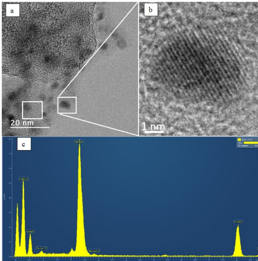
Figure 6. (a,b) HRTEM images and (c) EDX mapping image of the MOC10 sample.
