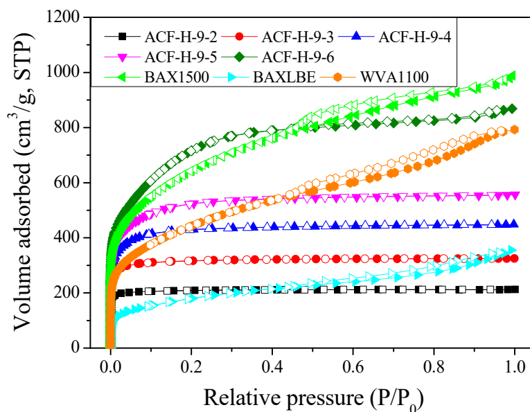
Figure 2. N_2/77\text{ K} adsorption–desorption isotherm curves of pitch-based activated carbon fibers as a function of various H_2O activation times and commercial activated carbons. ACF: activated carbon fibers.
