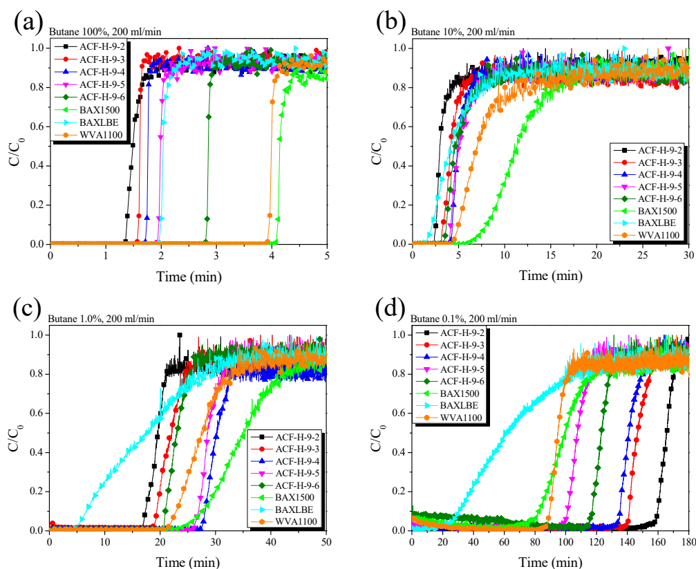
Figure 9. Breakthrough curves of pitch-based activated carbon fibers as a function of various H_2O activation time and butane concentration: (a) 100% butane, (b) 10% butane, (c) 1.0% butane, and (d) 0.1% butane.
