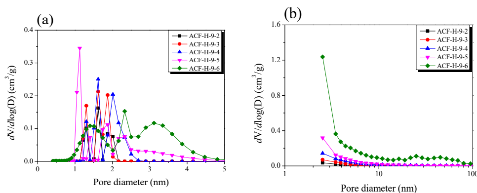
Figure 3. Pore size distribution of pitch-based activated carbon fiber as a function of various H 2 O activation time: (a) micropore size distribution by the nonlocalized density functional theory (NLDFT) method; (b) mesopore size distribution by the BJH equation.
