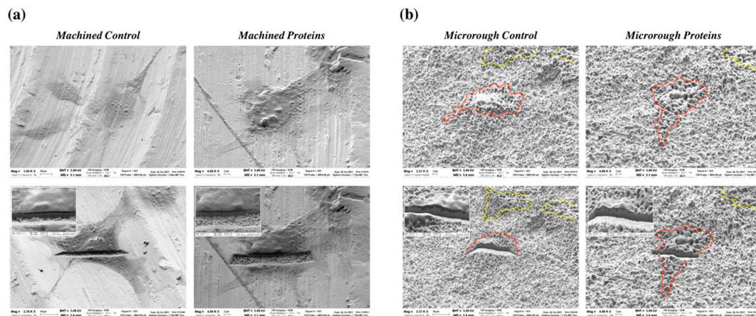
Figure 4. Scanning electron microscopy: (a) Representative SEM images showing MC3T3-E1 cells 24 h after seeding on machined titanium surfaces pre-conditioned or not with serum proteins, before and after focused ion beam (FIB) cross-sectional analysis; (b) representative SEM images showing MC3T3-E1 cells 24 h after seeding on microrough titanium surfaces pre-conditioned or not with serum proteins, before and after FIB cross-sectional analysis. Red and yellow lines highlight the borders of osteoblasts on titanium surfaces.
