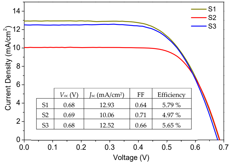
Figure 4. J - V curves for best devices fabricated using S1, S2, and S3 samples. The strong scattering effect within the TiO_2 layer in the S3 sample could almost retrieve the photocurrent of S1 made of monodispersed TiO_2 nanoparticles.
