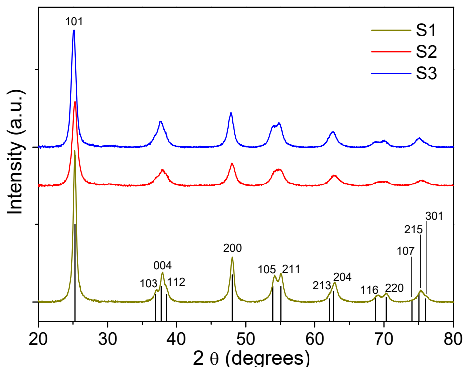
Figure 3. XRD patterns of samples S1, S2, and S3. All samples could be indexed with the JCPDS file No. 21-1272 for anatase TiO 2 structure, which is presented as black vertical bars at the bottom of the figure.
