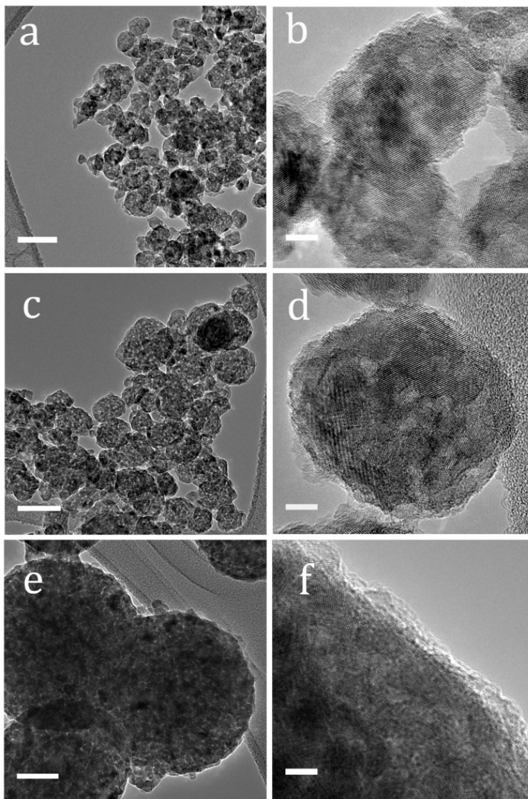
Figure 1. TEM and HRTEM images of sample (a, b) S1 (c, d) S2 (e, f) S3. The scale bars in the TEM images (a, c, e) correspond to 50 nm while the scale bars in the HRTEM images (b, d, f) correspond to 5 nm.
