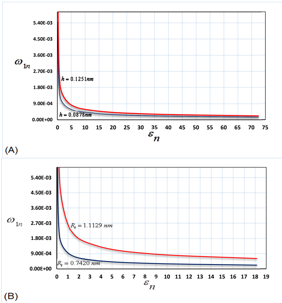
Figure 2. Nonlinear parameters versus frequency for the first mode of vibrations (A) h = 0.0878 \text{ nm} , h = 0.1251 \text{ nm} and (B) R_r = 0.7420 \text{ nm} , R_r = 1.1129 \text{ nm} .
