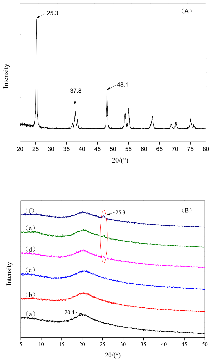
Figure 6. X-ray diffraction (XRD) analysis images for the morphology of original \text{TiO}_2 nanoparticles (A) and chitosan coating with \text{TiO}_2 nanoparticles (B) ( 10\text{ }\mu\text{m} \times 10\text{ }\mu\text{m} ; a: 0; b: 0.01%; c: 0.03%; d: 0.05%; e: 0.07%; f: 0.09%).
