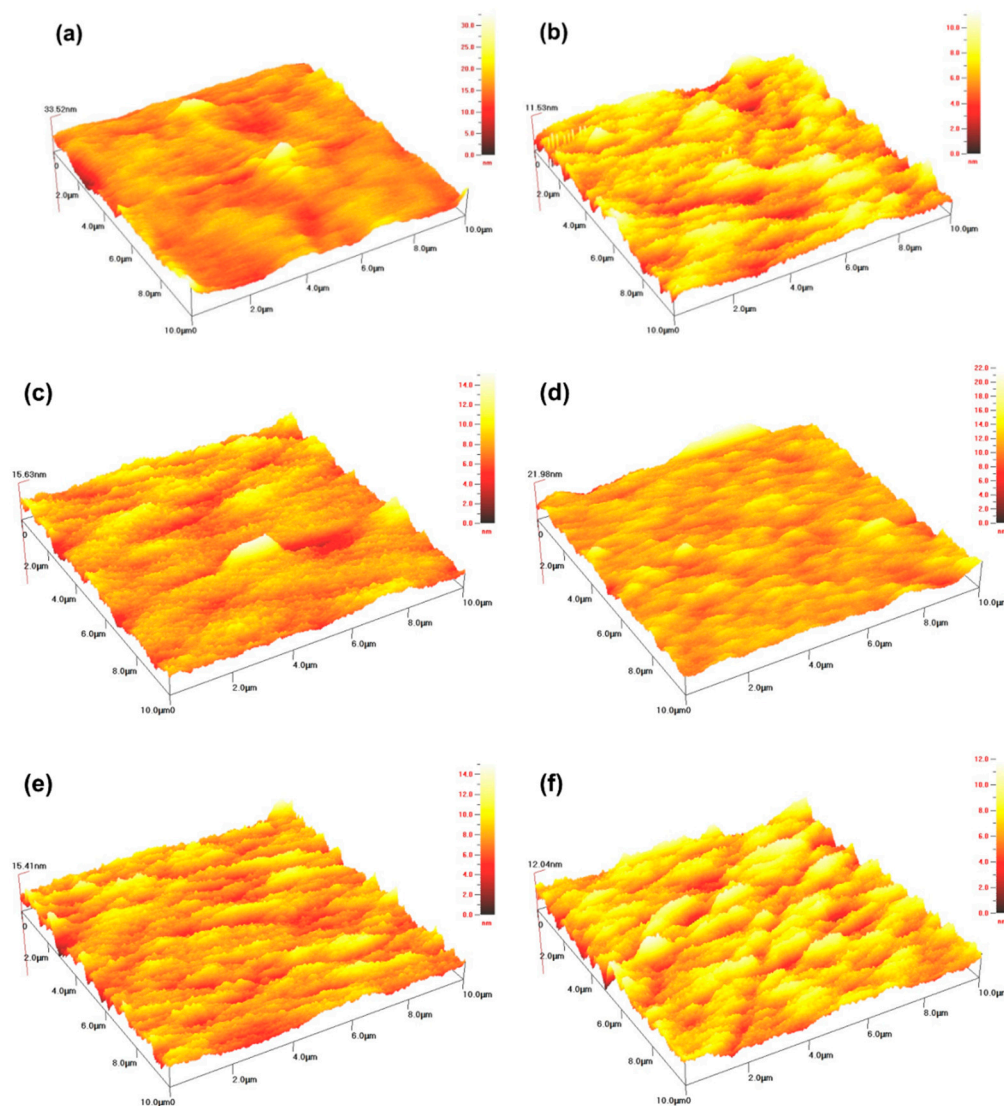
Figure 4. Atomic force microscopy (AFM) analysis images for the morphology of chitosan coating with \text{TiO}_2 nanoparticles 10\ \mu\text{m} \times 10\ \mu\text{m} ; (a) 0; (b) 0.01%; (c) 0.03%; (d) 0.05%; (e) 0.07%; (f) 0.09%.
