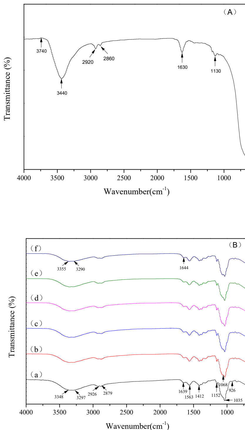
Figure 7. Fourier transform infrared spectroscopy (FTIR) spectra of original TiO 2 nanoparticles (A) and chitosan-based coating with different concentrations of TiO 2 nanoparticles (B) (a: 0; b: 0.01%; c: 0.03%; d: 0.05%; e: 0.07%; f: 0.09%).
