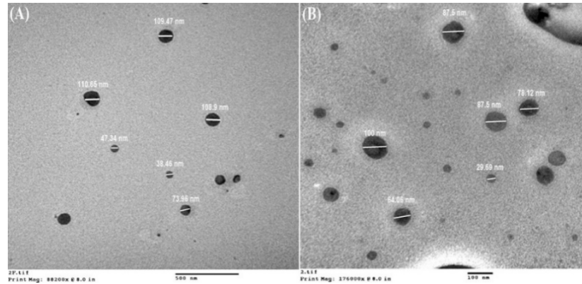
Figure 6. TEM images of CPN, subfigure (A) represents particles size at 500 nm scale and subfigure (B) represents particles size at 100 nm scale
