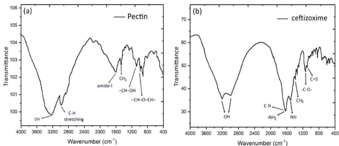
Figure 3. FTIR spectra of pectin (a) and ceftizoxime (b).
