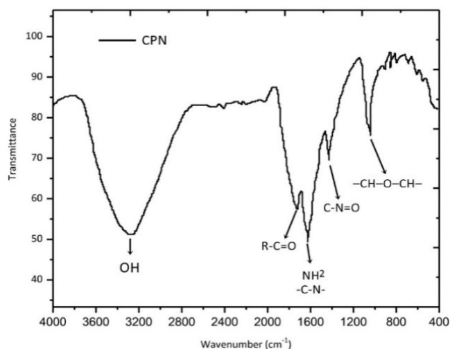
Figure 4. FTIR spectra of CPN.
