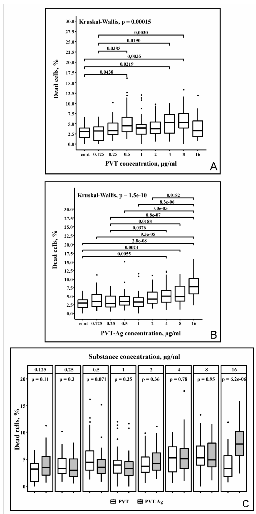
Figure 8. Analysis of the number of dead fibroblasts after incubation for 24 h with (A) PVT, (B) Ag(0)-PVT in the different concentrations and (C) in comparison to each other.. Medians, first and third quartiles are presented; p -values are given only for significant differences ( p < 0.05 ).
