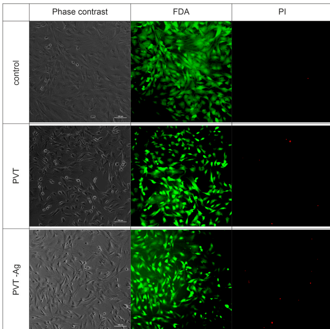
Figure 7. Incubation with fibroblasts for 24 h: control, PVT 16 \mu\text{g/mL} , AgNPs nanocomposites (PVT-Ag) 16 \mu\text{g/mL} . Phase contrast, fluorescence staining with fluorescein diacetate (FDA) (green) and propidium iodide (PI) (red). Scale bars 100 \mu\text{m} .
