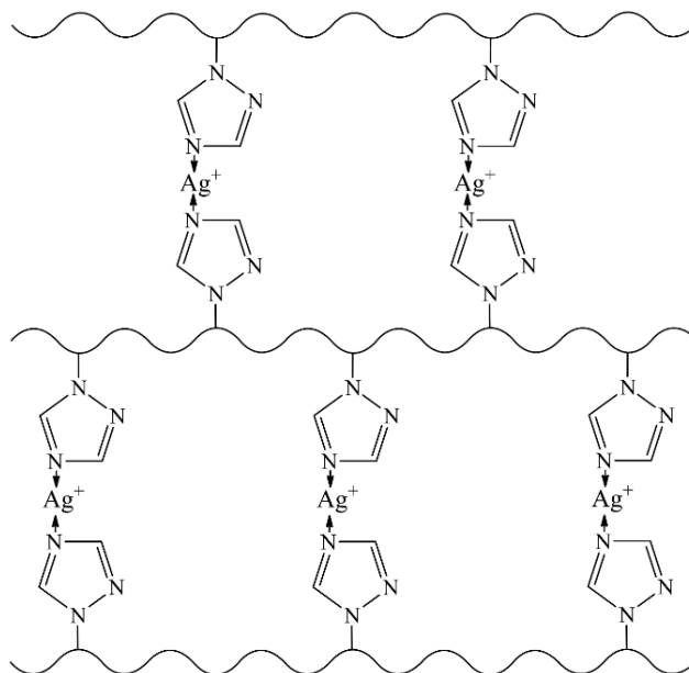
Figure 2. Schematic coordination interaction of silver ions with PVT macromolecules.
