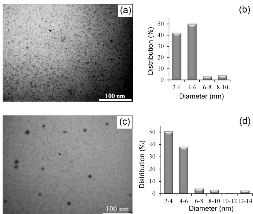
Figure 5. (a,c) TEM images and (b,d) sizes histograms of AgNPs nanocomposites synthesized using various different reducing agents. (a,b) NaBH 4 and (c,d) formaldehyde.
