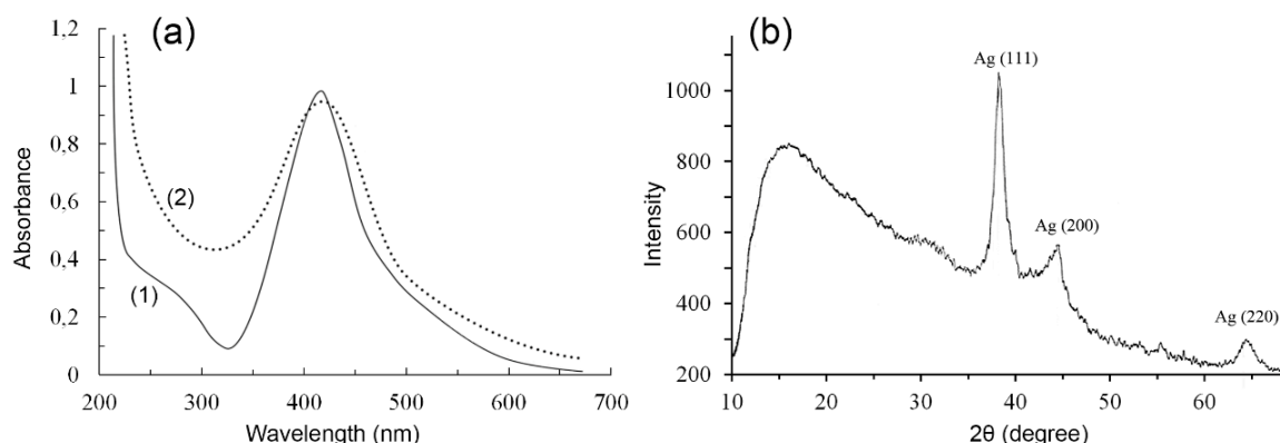
Figure 4. (a) UV-visible spectra of AgNPs nanocomposites synthesized using various different reducing agents: NaBH 4 (1) and formaldehyde (2); (b) typical X-ray diffraction pattern of AgNPs nanocomposites.
