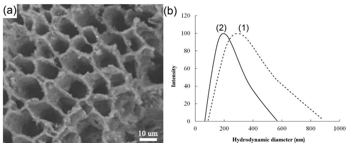
Figure 1. (a) SEM image of PVT and (b) particle size distribution curves of the (1) initial PVT and (2) AgNPs nanocomposite.
