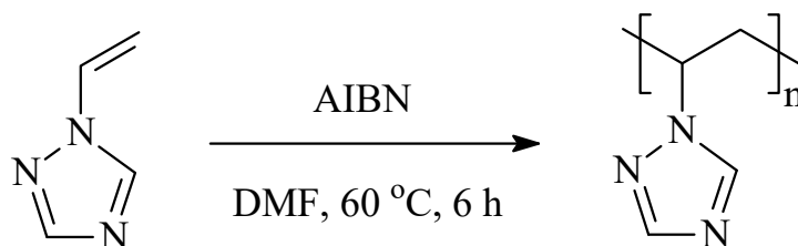
Scheme 1. Synthesis of poly-1-vinyl-1,2,4-triazole (PVT).
