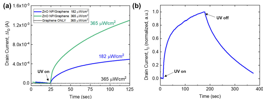
Figure 8. Temporal photoresponse of ZnO nanoparticle/graphene devices: (a) ZnO nanoparticle/graphene device compared with the graphene only device at 182 \mu\text{W}/\text{cm}^2 and 365
