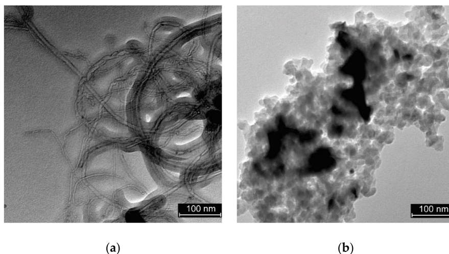
Figure 1. Transmission electron microscopy (TEM) images of: (a) molybdenum carbide supported on carbon nanotubes ( \text{Mo}_2\text{C}/\text{CNT} ) and (b) molybdenum carbide supported on carbon xerogel ( \text{Mo}_2\text{C}/\text{CXG} ).
