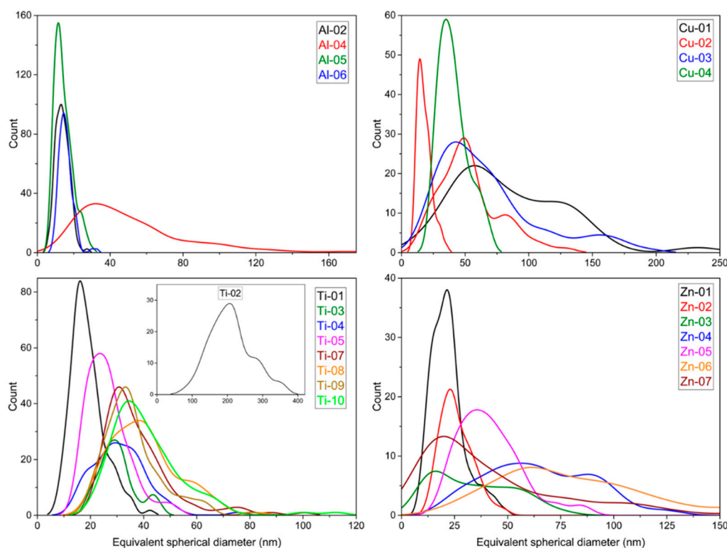
Figure 5. Smooth histogram plots illustrating the distributions for the equivalent spherical diameter for the various metal oxides. Two plots (Feret and minFeret in red) are shown for the nanorod sample, Cu-02. The insert in the bottom left plot shows the Ti-02 histogram on a larger x -axis scale.
