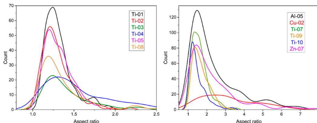
Figure 6. Smoothed histogram plots for aspect ratio for representative metal oxides nanomaterials. \text{TiO}_2 samples with mean aspect ratios < 1.5 are shown in the left panel and several samples with higher mean aspect ratios are shown in the right panel.
