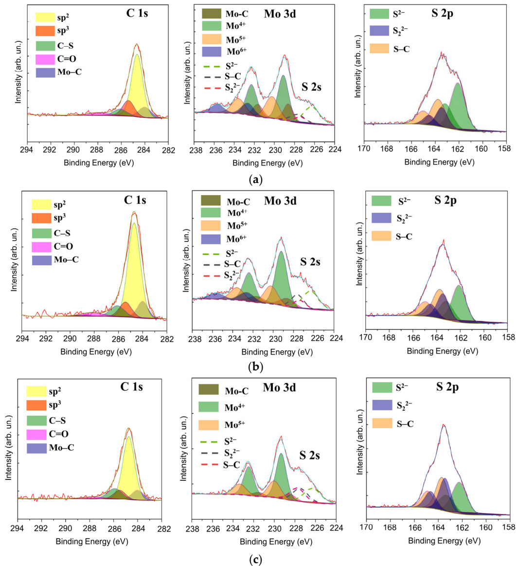
Figure 7. XPS spectra of C 1s, Mo 3d, and S 2p which were measured on the surface of the Mo–S–C–H thin-film coatings obtained by reactive PLD at H_2S pressures of (a) 5.5, (b) 9, and (c) 18 Pa. For Mo 3d spectra, the S 2s spectra of different S species are indicated.
