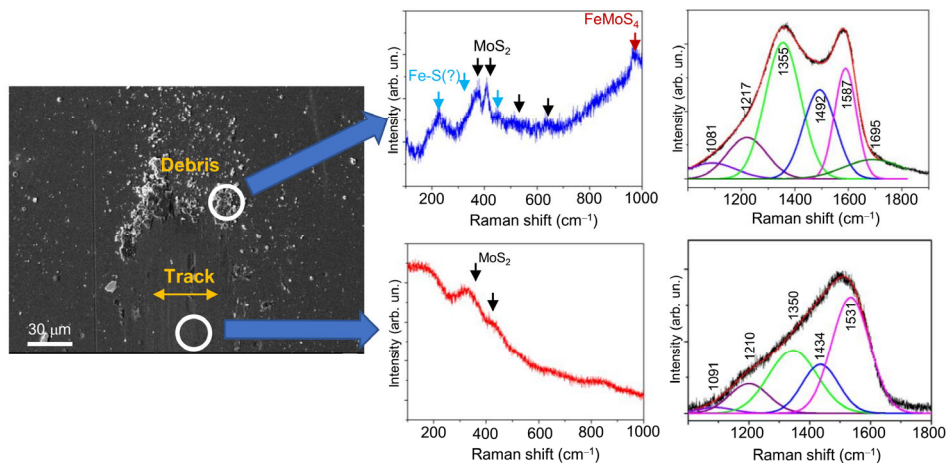
Figure 15. SEM image and Raman spectra for the Mo-S-C-H 5.5 thin-film coating subjected to pin-on-disk test at 22 °C in dry friction conditions (RH ~8%).
