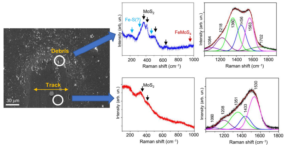
Figure 14. SEM image and Raman spectra for the Mo-S-C-H 5.5 thin-film coating subjected to pin-on-disk test at 22 °C in wet friction conditions (RH ~58%).
