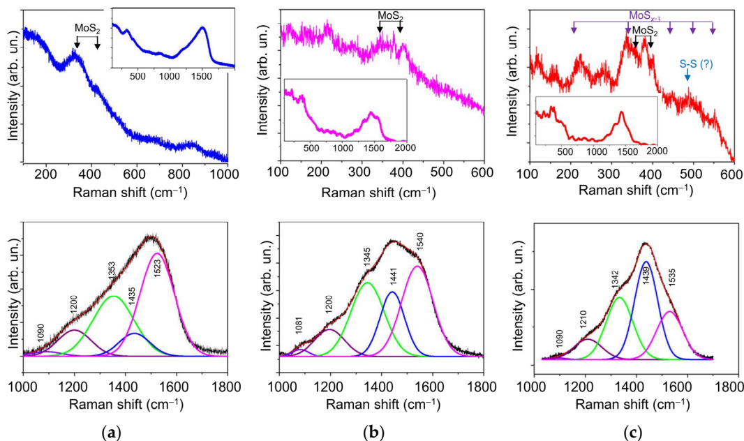
Figure 6. Raman spectra for the Mo-S-C-H thin-film coatings obtained by reactive PLD in the H 2 S gas at pressures of (a) 5.5, (b) 9, and (c) 18 Pa. The regions of Raman shifts corresponding to resonance light scattering by MoS x - and a-C(S,H)-based nanophases are shown at the top and bottom, respectively. The model of spectrum decomposition into the indicated peaks is discussed in the text. Inserts show the Raman spectra in the region from 100 to 2000 cm -1 that allows a correct comparison of the peak intensities for different nanophases.
